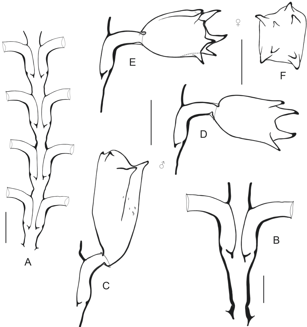
Fig. 8. Synthecium brucei Vervoort & Watson, 2003. Portion of colony (A). Hydrothecal pair, enlarged (B). Various gonothecae seen laterally (C-E), the latter also in apical view (F). Scale bars: 500 \mu m (B), 1 mm (A, C-F).
