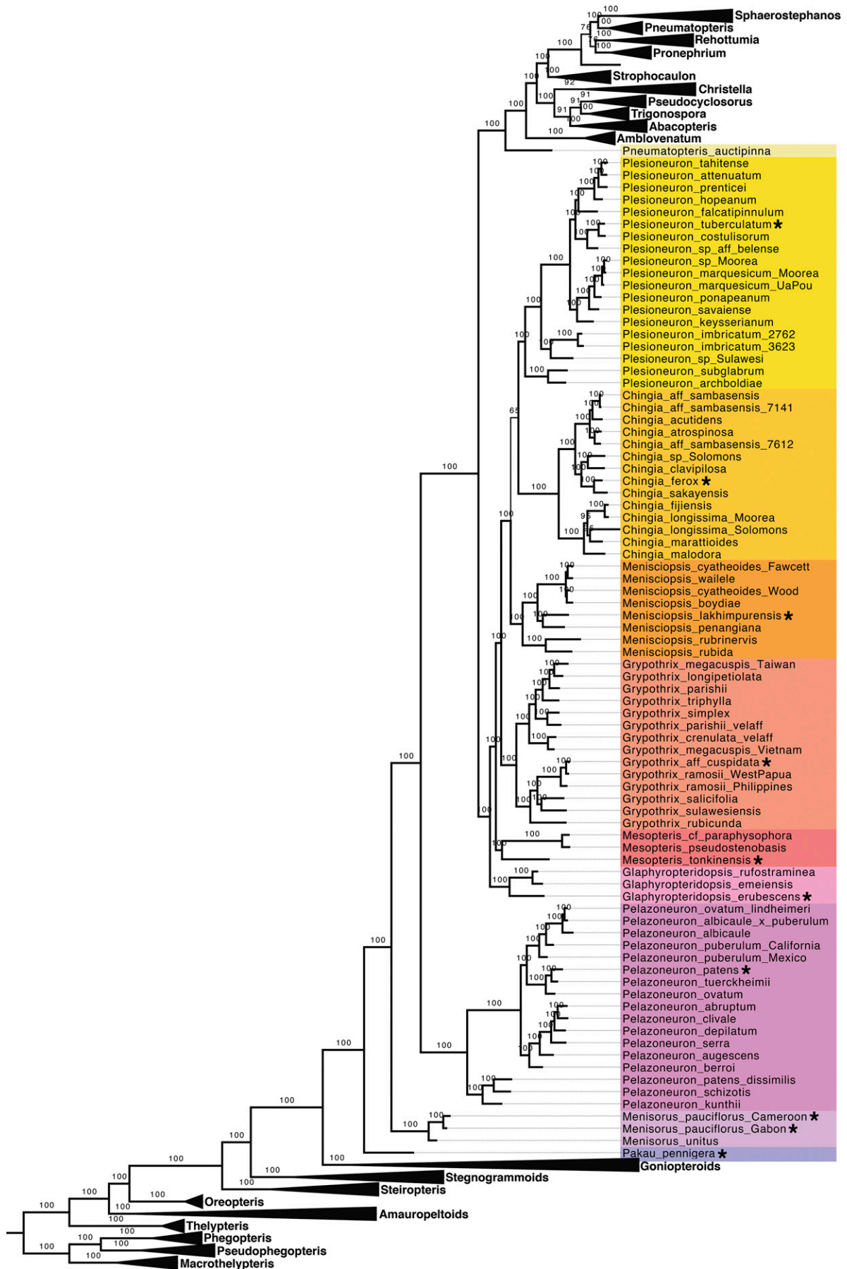
FIG. 3F. The monotypic genus Pakau , and the members of the chingioideae in the maximum likelihood phylogeny of the 407-locus concatenated alignment. The nodes are annotated with ultrafast bootstrap support values, and genera are emphasized by distinct colors. Type species of genera are denoted with an asterisk (*).
