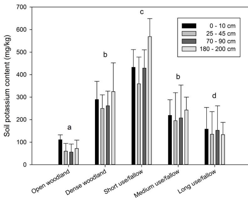
Fig. 6. Soil potassium content of the vegetation categories for different soil depths. Whiskers display standard deviation; letters indicate significant differences between categories with p < 0.05 according to Mann-Whitney pairwise comparisons.
