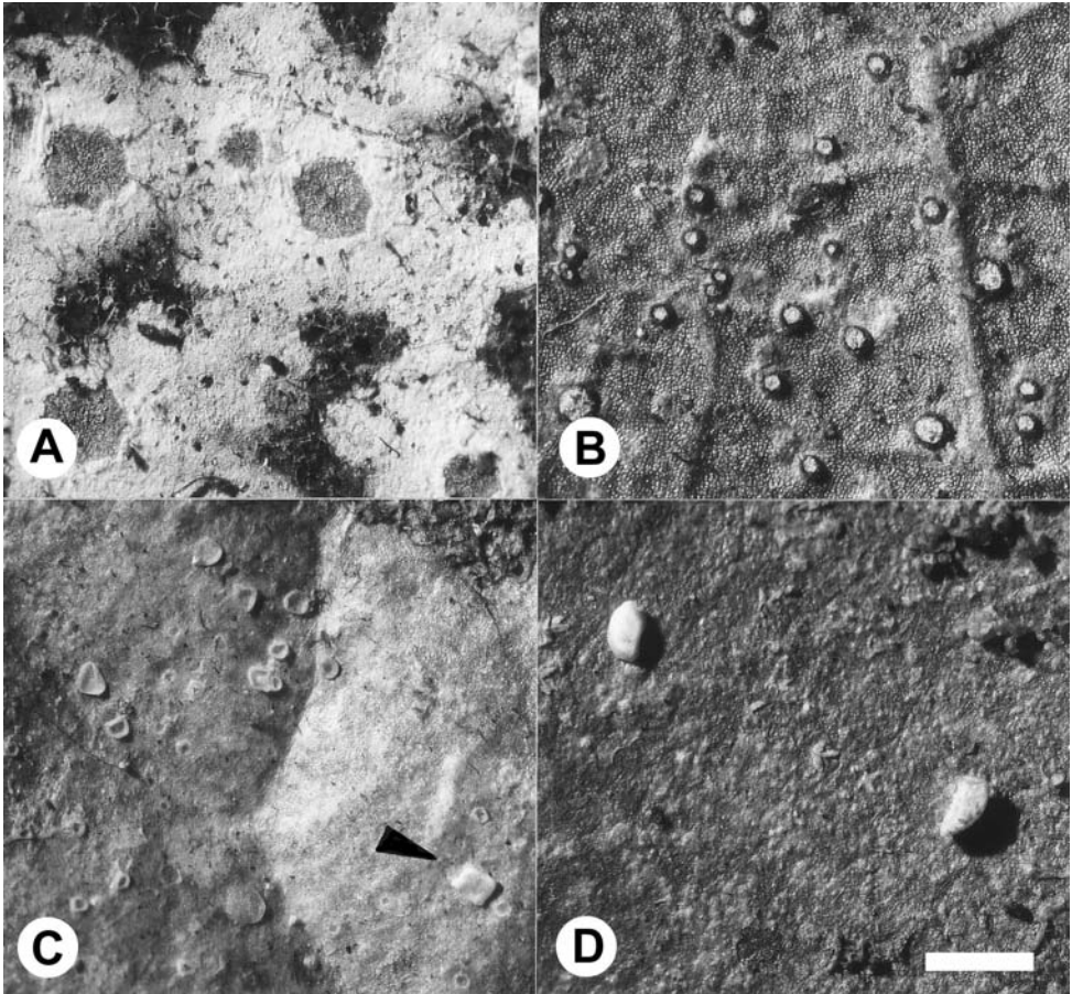
Fig. 4. A: Echinoplaca aff. atrofusca R. Sant., thallus with apothecia; B: Gyalideopsis albopruinosa Lücking, thallus with apothecia; C-D: Gyalideopsis hyalina Lücking, thallus with apothecia and campylidioid hyphophores (arrow). – Scale = 1 mm.
