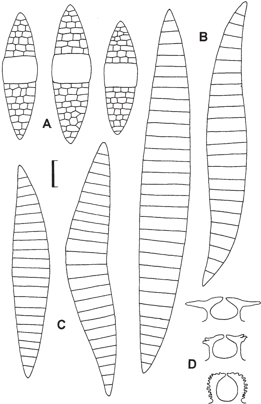
Fig. 2. A: Aspidothelium mirabile Lücking, ascospores; B: A. ornatum Lücking, ascospores; C: A. scutellarpum Lücking, ascospores; D: schematic section through perithecia in A. scutellarpum (above), A. fugiens (Müll. Arg.) R. Sant. (middle) and A. ornatum (below). – Scale = 10 µm for ascospores and 200 µm for perithecial sections.
