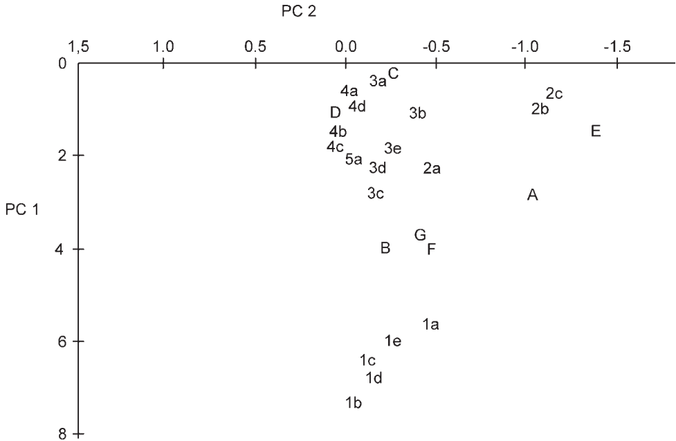
Fig. 10. PCA – plot of the first two principal components (PC1 and PC2).
