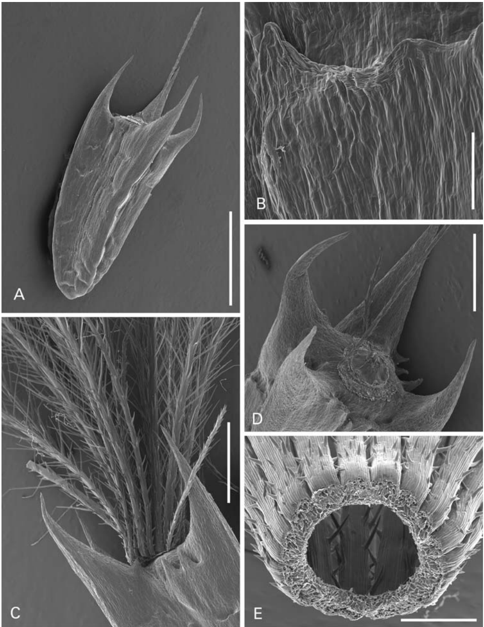
Fig. 4. Lipschitziella ceratocarpa , scanning electron micrographs of achenes and pappus (from Lace 1789) – A: overview; B: surface; C: pappus detail; D: apical region; E: base of inner pappus. – Scale bars A = 2 mm, B = 0.09 mm, C = 0.9 mm, D = 0.8 mm, E = 0.3 mm.
