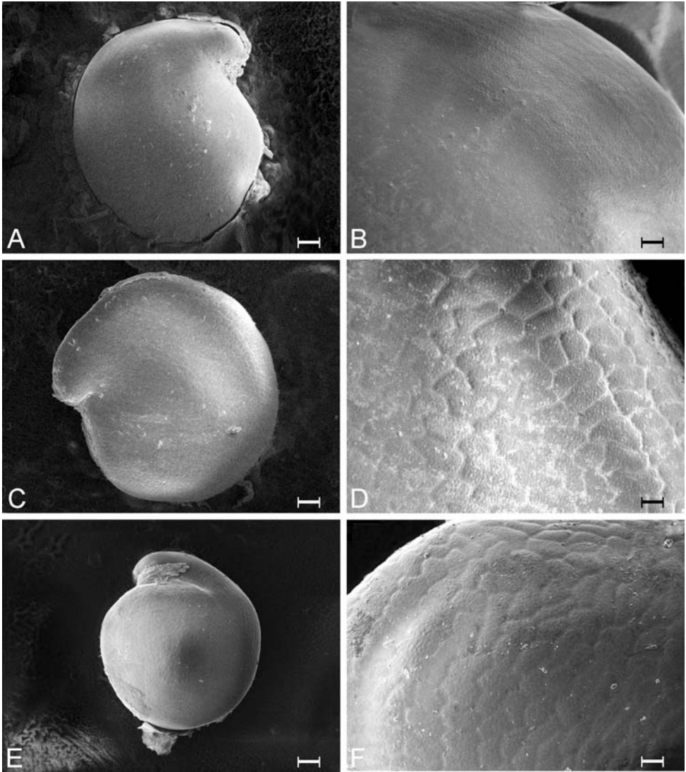
Fig. 7. SEM photographs of Suaeda seeds – A-B: S. crassifolia (from the lectotype); C-D: S. salsa (from the epitype); E-F: S. prostrata (from the epitype). – Scale bars A, C, E = 100 µm, B, D, F = 20 µm; photographs by M. Lomonosova and Y. Lukjanov.
