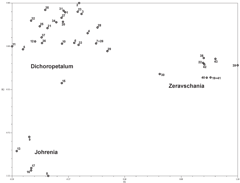
Fig. 4. Two-factor plot (components 1 and 2) showing OTUs relationships in reduced character space. Downloaded From: https://bioone.org/journals/Willdenowia on 30 Apr 2024 Terms of Use: https://bioone.org/terms-of-use
