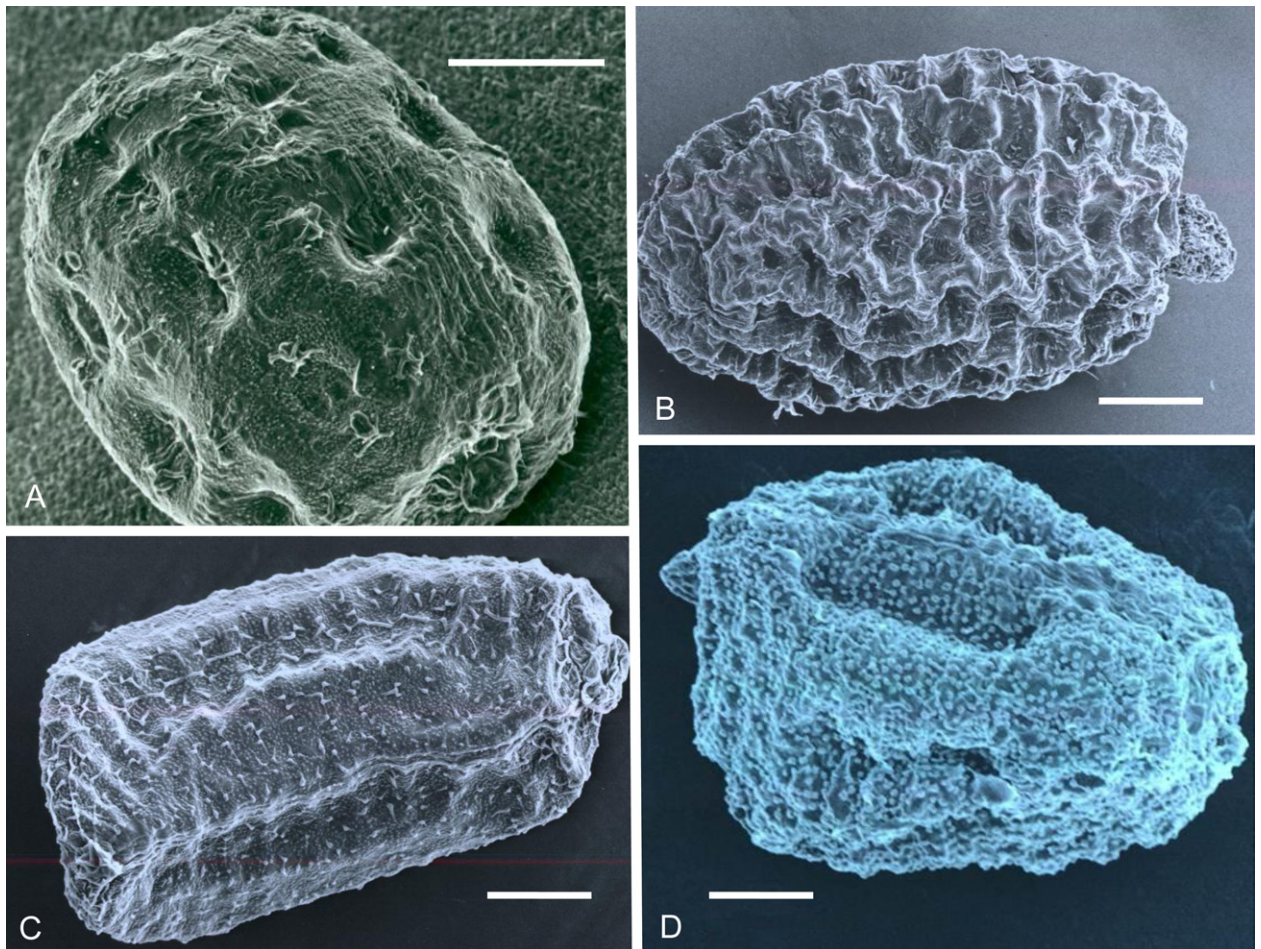
Fig. 3. SEM photographs of Linderniaceae seeds – A: Torenia crustacea ; B: Linderniella cerastioides ; C: Lindernia rotundifolia ; D: Crepidorhopalon microcarpaeoides . – Scale bar 100 \mu\text{m} . – Photographs by E. Fischer.
