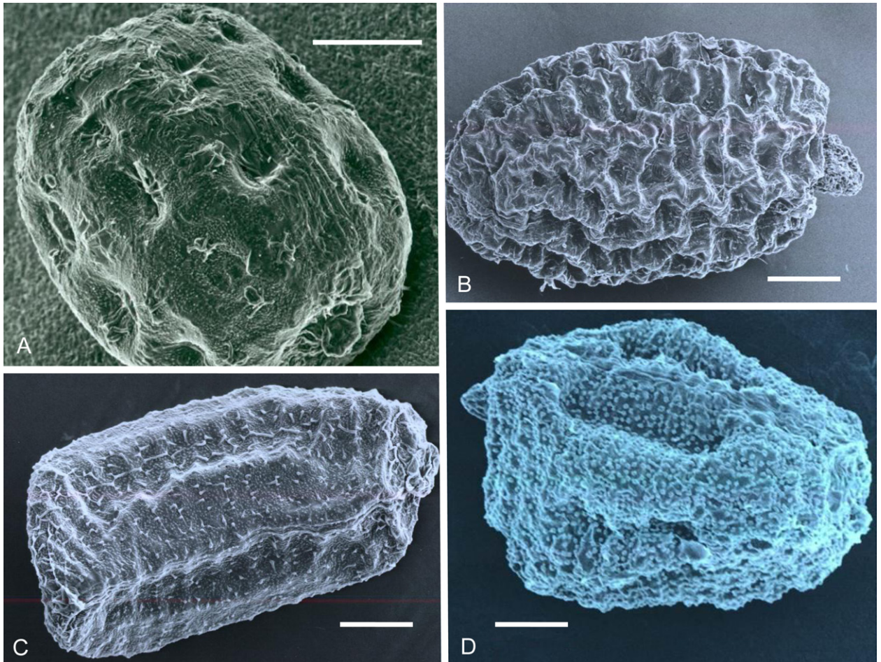
Fig. 3. SEM photographs of Linderniaceae seeds – A: Torenia crustacea ; B: Linderniella cerastioides ; C: Lindernia rotundifolia ; D: Crepidorhpalon microcarpaeoides . – Scale bar 100 \mu m. – Photographs by E. Fischer.
