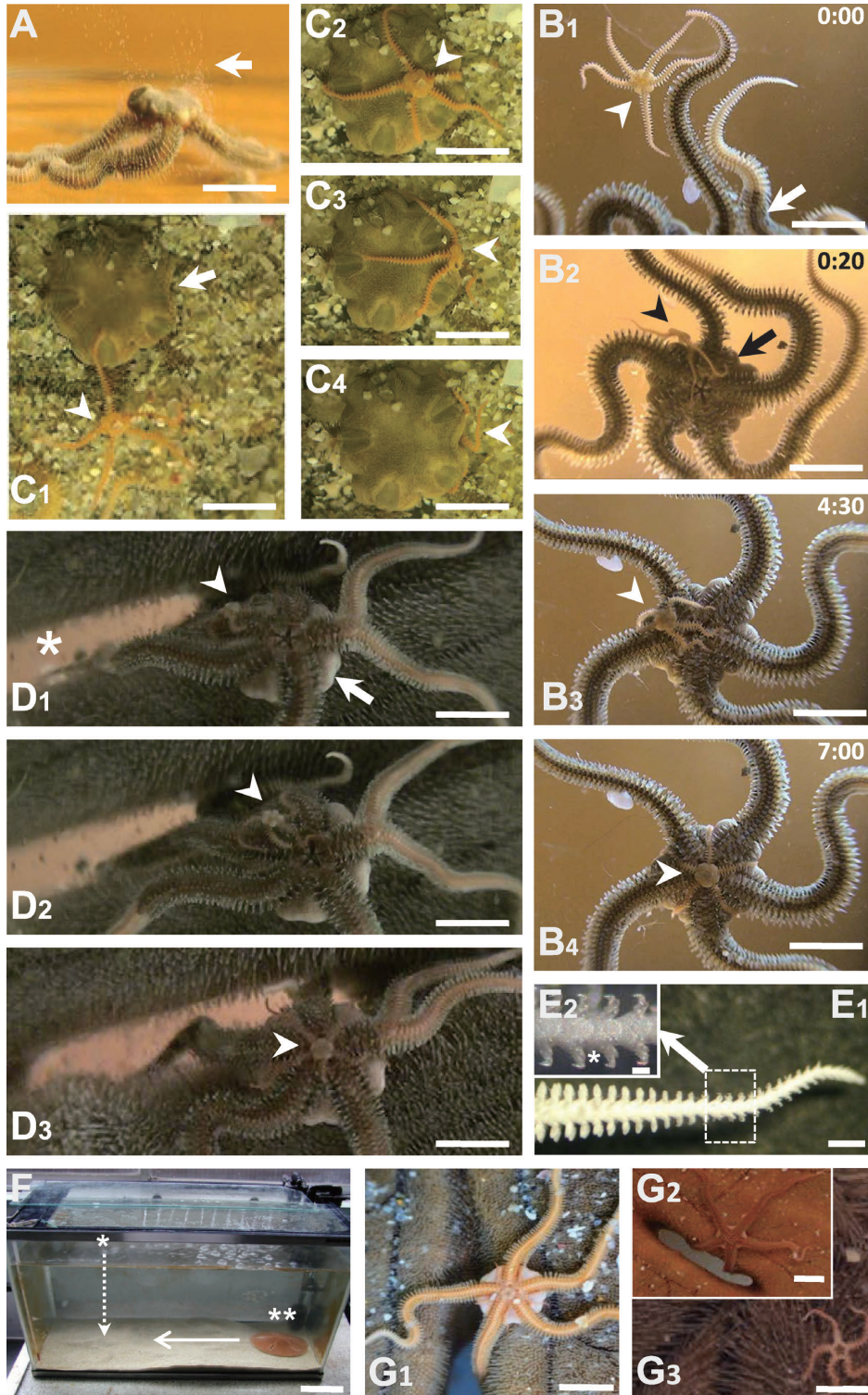
Fig. 3. Spawning, coupling, and attachment behaviors of O. formata . (A) Spontaneous shedding posture of coupled ophiuroids. Spawning eggs are visible (arrow). (B) The overall style of coupling behavior between a female (arrows) and a male (arrowheads), viewed from below the glass vessel. The dwarf male approaches a solitary female ( B 1 ), becomes attached to the female's disk, and rotates his disk vertically ( B 2 ). The male holds the larger female, with the oral surfaces of the two sexes closely appressed ( B 3 ). Note the male's position, with five arms situated at the interradius of the female ( B 4 ). (C) Coupling behavior between a female (arrow) and a male (arrowheads) on sand, viewed from above. The dwarf male approaches the female ( C 1 ), climbs onto the female's disk ( C 2 ), and rotates his disk vertically ( C 3-4 ) in the same way as shown in (Fig. 3, B 1-2 ). (D) Coupling behavior between a female (arrow) and a male (arrowheads) on the oral surface of their host, the sand dollar Astriclypeus manni , in a water tank viewed from below. The dwarf male waits for a female at the external edge of the lunule (asterisk) of his host, approaches ( D 1 ), and becomes attached to the female's oral surface ( D 2-3 ) in the same way as in (Fig. 3, B 3-4 ). Oral views (female) and aboral views (male). (E) Aboral view of the hook-shaped arm spines at the tips of a female's arm. Note that four pairs of spines ( E 2 ; asterisk) are directed aborally at the base of the rectangular part surrounded by dotted lines ( E 1 ). (F) The water tank equipment used for observing the attachment behavior of O. formata . An ophiuroid was dropped onto the bottom (asterisk and dashed arrow), and its attachment behavior to the host was then recorded. Arrow (solid line) indicates the direction of movement of the host A. manni (double asterisks). (G) Position of ophiuroids on a host. Note the pair of coupled ophiuroids ( G 1 ), a solitary female ( G 2 ), and a solitary male ( G 3 ) attached to the margin of the lunule and the oral surface of the host, respectively. Arabic numerals on the upper right ( B 1-4 ) indicate the elapsed time (minutes and seconds). Scale bars: (A, B 1-4 , C 1-4 , D 1-3 , G 1-2 ) 5 mm, (E 1 , G 3 ) 1 mm, (E 2 ) 500 \mu\text{m} , (F) 10 cm.
