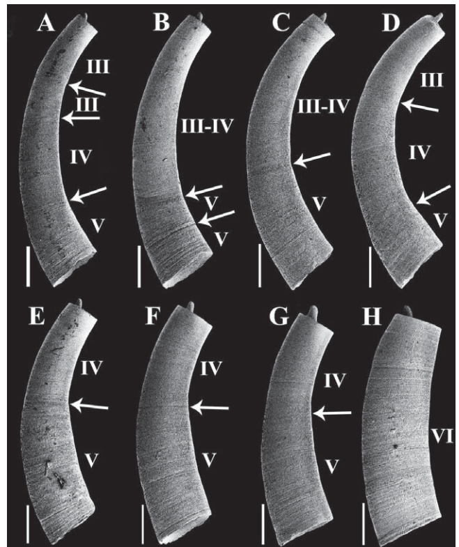
Fig. 8. Caecum trinidadense sp. nov. shells at different growth stages (paratypes: IBUFRJ 19599): (A–D) teleoconch III to V; (E–H) teleoconch IV to VI. Scale bars: 500 \mu m.
