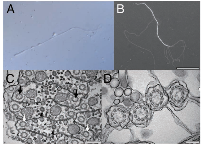
Fig. 4. Sperm of Amphiscolops oni sp. nov. (A) Light microscopy and (B) scanning electron microscopy of the sperm. (C) Transmission electron micrograph of the shaft section of a bundle of sperm. A pair of axonemes present in a single sperm is shown with black and white arrows, respectively. Black arrowheads: axial microtubules. (D) Transmission electron micrograph of axonemes of sperm. Lack of central singlet microtubules in the axonemes can be seen. Both outer and inner dynein arms are observed. Scale bars: 20 \mu m (B); 500 nm (C); 200 nm (D).
