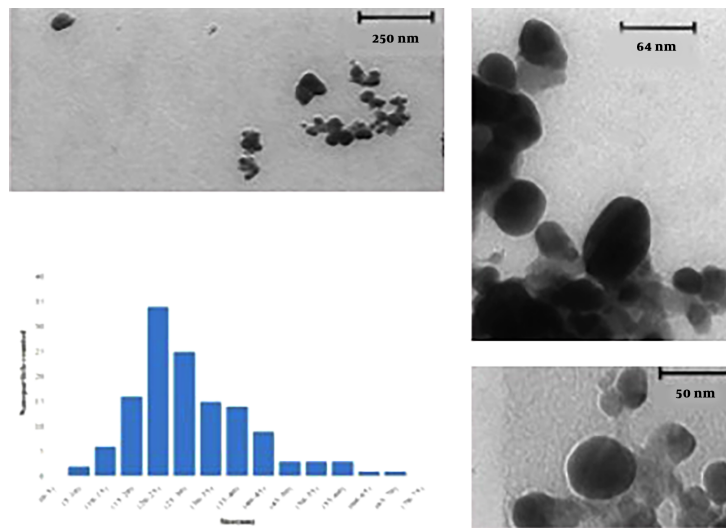
Figure 4. TEM images of area of a drop-coated film of silver nanoparticles biosynthesized by endophytic fungal isolate
