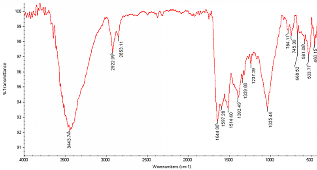
Figure 5. FTIR spectrum of silver nanoparticles, synthesized by endophytic fungal isolate
