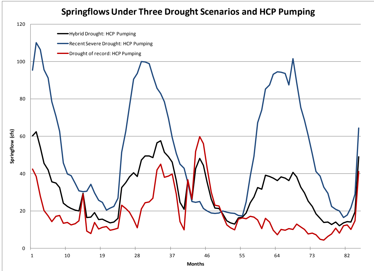
Figure J-3. Development of the Hybrid Drought from the DOR and Recent Severe Droughts.
