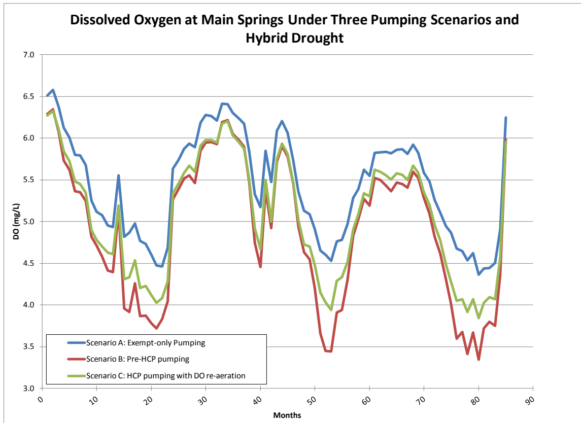
Figure J-4. Dissolved Oxygen at Main Spring under the various management scenarios during Hybrid Drought conditions. The HCP does not take into account the benefits of the COA’s planned DO re-aeration from spring-run improvements (+0.3 mg/L), nor any proposed mitigation.
