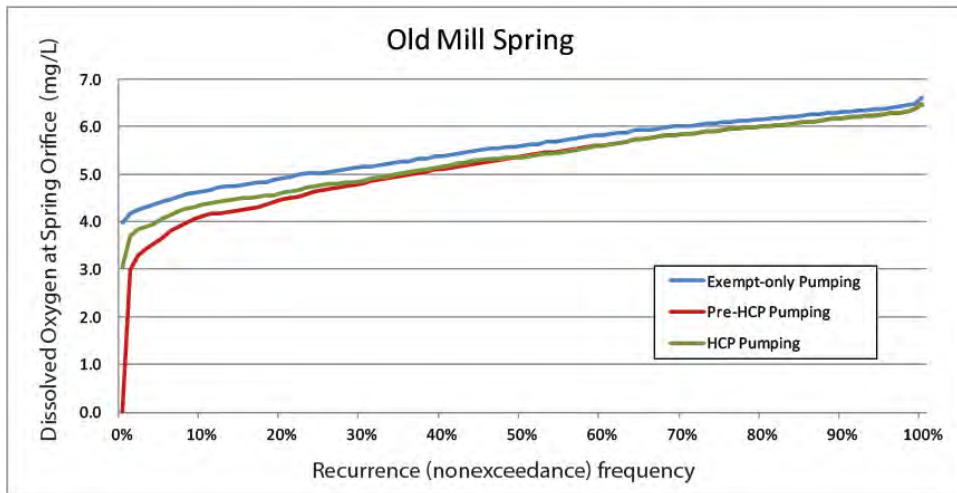
Figure J-2(a-c). Non-exceedance frequency of dissolved oxygen concentration for the period of record at Main, Eliza, and Old Mill Spring under three groundwater management scenarios. The correlations of springflow to DO are derived from Porrás(2014). These curves do not reflect the benefits of the mitigation measures.
