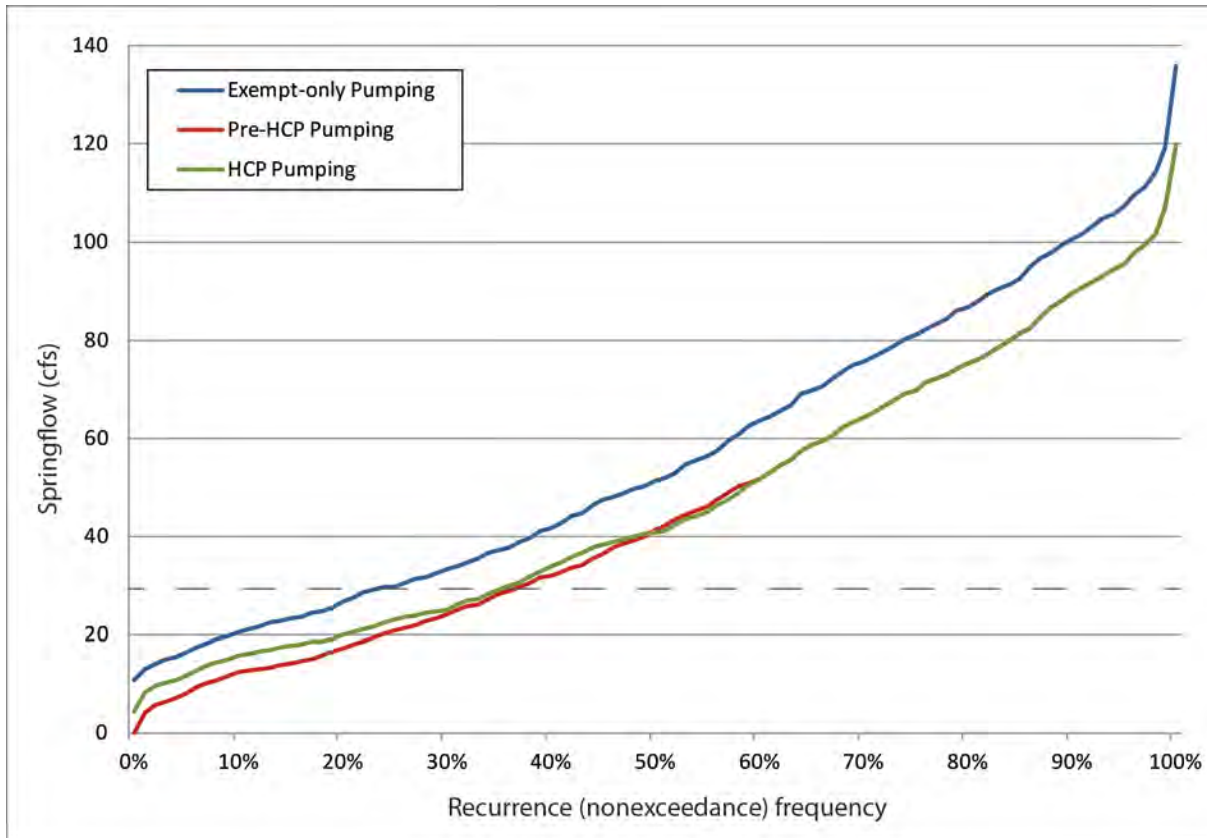
Figure J-1. Recurrence (non-exceedance) frequency of Barton Springs flow for the period of record under three groundwater management scenarios.
