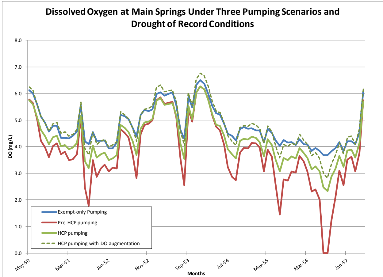
Figure J-5. Dissolved Oxygen at Main Springs under the various management scenarios during Drought of Record conditions. The solid lines do not include any mitigation measures. The dashed HCP line illustrates the effect of a modest amount of DO augmentation (at +0.5 mg/L DO) as proposed mitigation, improving estimated DO levels relative to the exempt-only pumping scenario.
