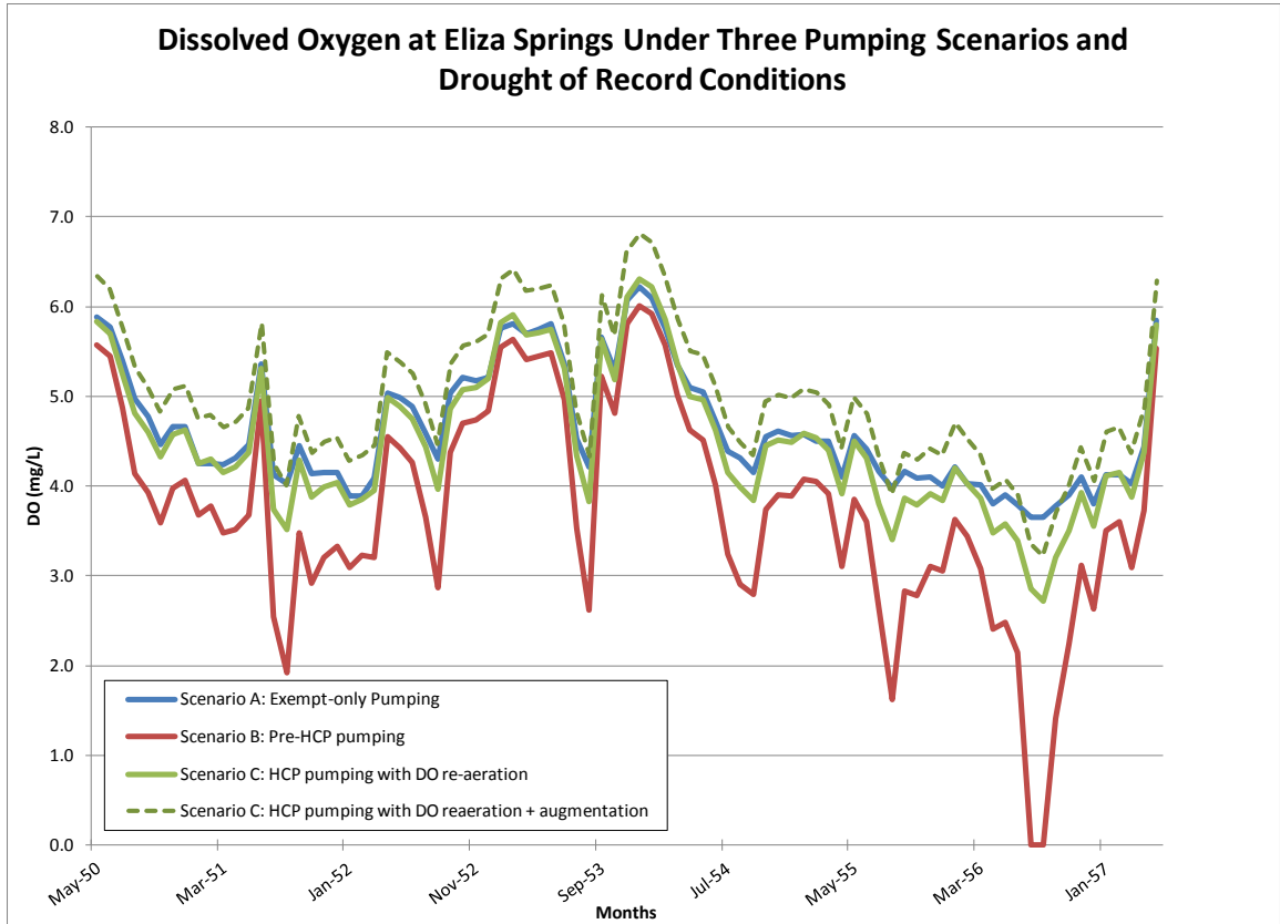
Figure J-6. Dissolved Oxygen at Eliza Spring under the various management scenarios during Drought of Record conditions. The solid HCP line takes into account the benefits of the COA’s planned DO re-aeration from spring-run improvements (+0.3 mg/L), and the dashed HCP line illustrates the effect of a modest amount of DO augmentation (at +0.5 mg/L DO) as proposed mitigation, improving estimated DO levels relative to the exempt-only pumping scenario.
