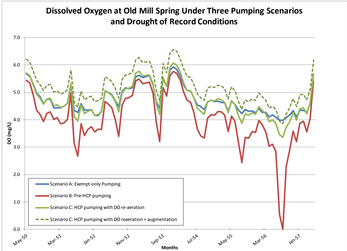
Figure J-7. Dissolved Oxygen at Old Mill Spring under the various management scenarios during Drought of Record conditions. The solid HCP line takes into account the benefits of the COA’s planned DO re-aeration from spring-run improvements (+0.3 mg/L), and the dashed HCP line illustrates the effect of a modest amount of DO augmentation (at +0.5 mg/L DO) as proposed mitigation, improving estimated DO levels relative to the exempt-only pumping scenario.
