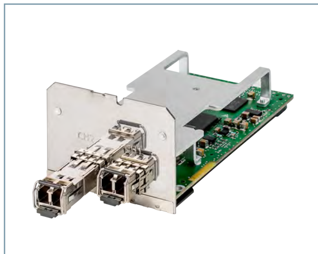
Figure 3.7/7 Optical Ethernet Module (ETH-BD-2FO)
