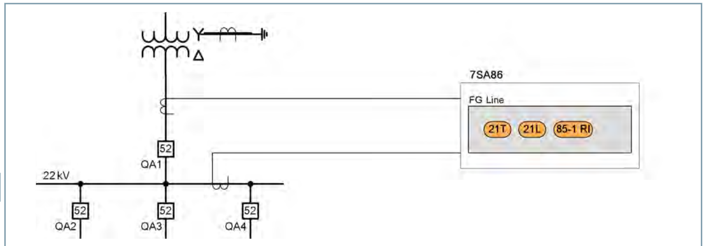
Figure 2.3/25 Impedance Protection
