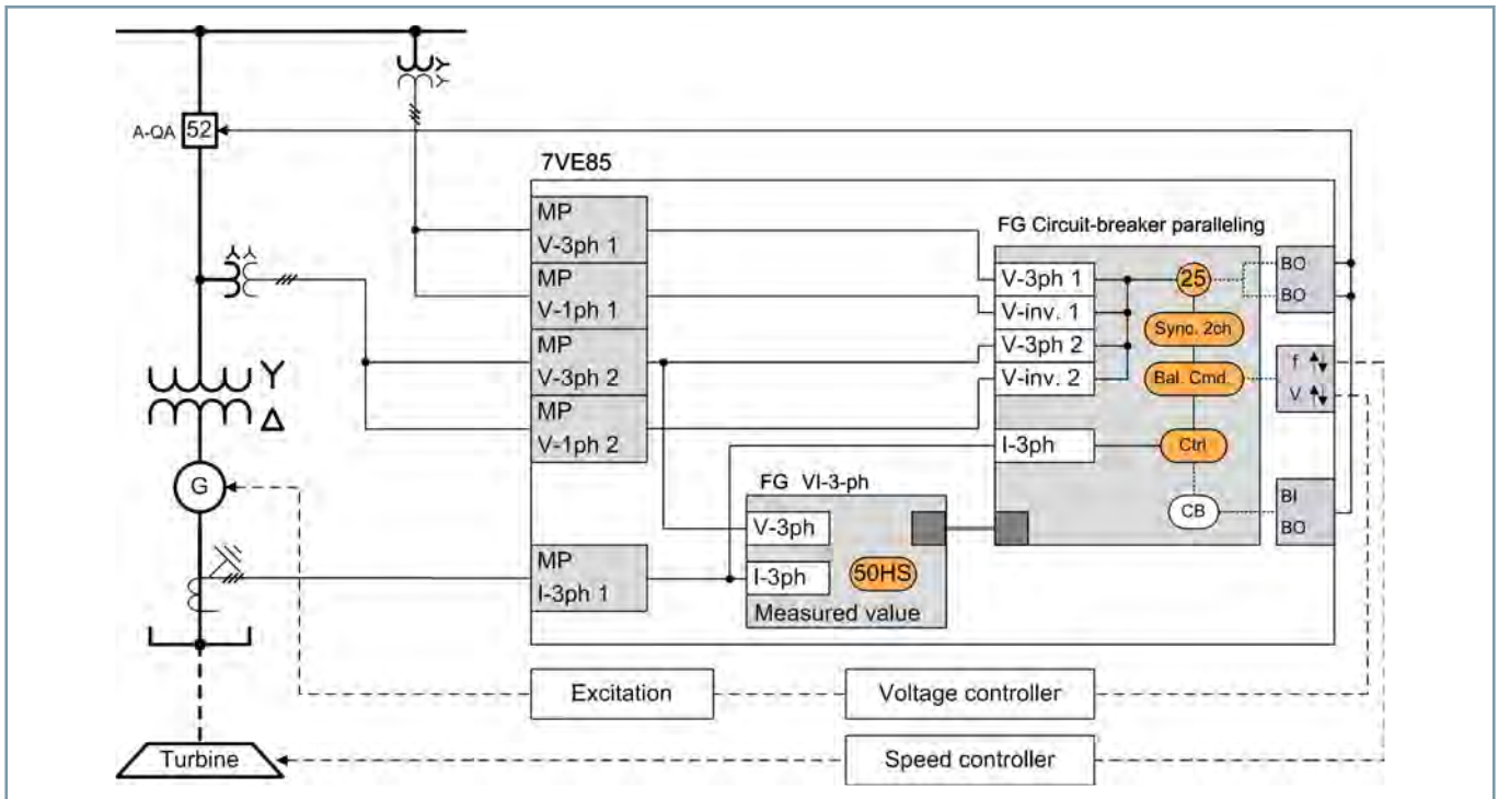
Figure 2.14/6 Application Template: Paralleling Extended 2 Channels with Balancing Commands 8 V, 8 I
