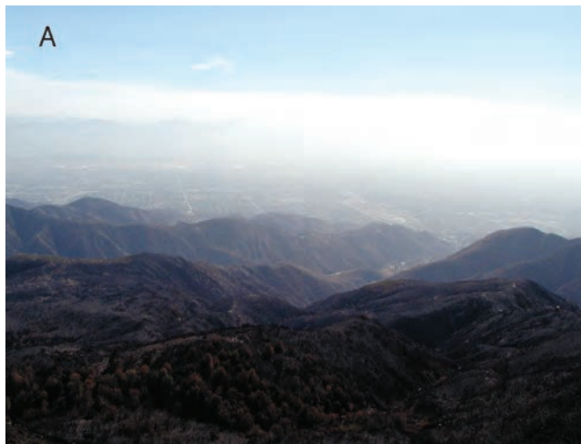
Photochemical smog. A Over the Los Angeles Basin, view from the San Bernardino Mountains. Photo: Andrzej Bytnerowicz. B Over the San Joaquin Valley, view from Moro Rock. Photo: Andrzej Bytnerowicz.
