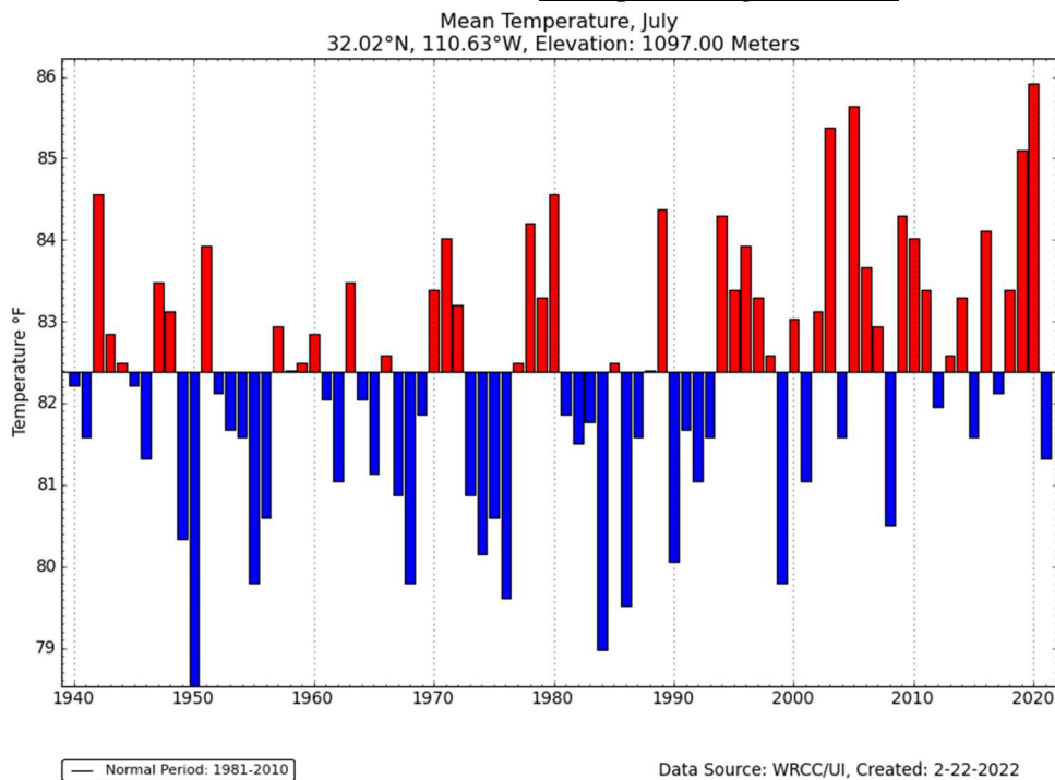
Figure 4. Mean July temperatures for the Cienega Creek Natural Preserve from 1940-2021, plotted to emphasize difference from long-term average of 82.4° F. July mean temperatures prior to 1995 were cooler than afterwards.
