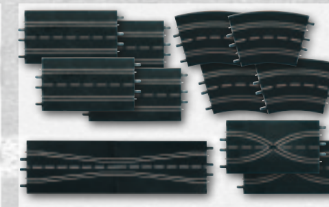
26956 Carrera DIGITAL 132 · Evolution Extension Set · 4 standard straights, 2 lane change sections, 2 chicane, 4 curves 2/30°, track section bolts
