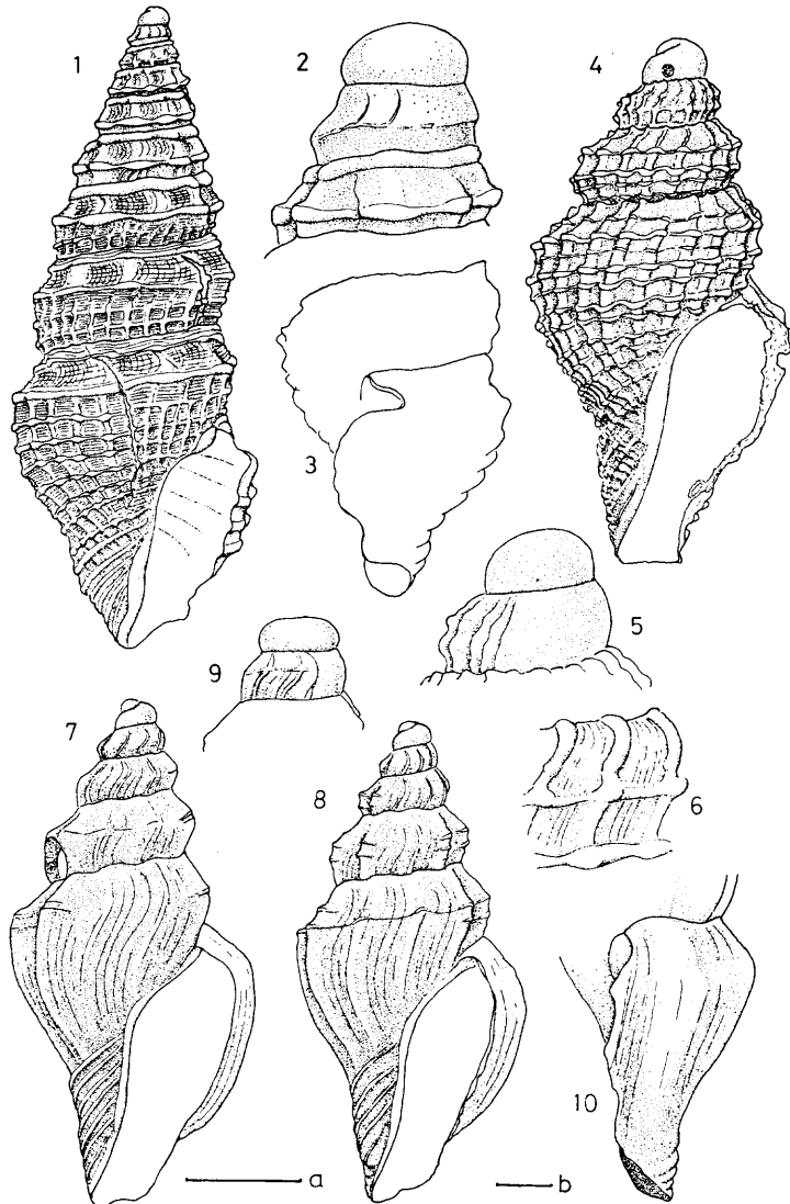
Fig. 3. Australian turrids 1-3. Paradrillia (Paradrillia) darnleyensis sp. nov. holotype, C 61502, front view (1), protoconch (2) and body whorl showing anal sinus (3). 4-6. Euryentmena australiana sp. nov. holotype, C 134678, front view (4), protoconch (5) and sculptural pattern on the upper part of the body whorl (6). 7-10. Anti-guraleus stellatomoides sp. nov. holotype, C 134686a, front view (7) and anal sinus (10); paratype, C 134686b, front view (8) and protoconch (9). Scale bar a 1 mm for 4 and 9; 0.5 mm for 2, 5 and 6. Scale bar b 1 mm for 1, 3, 7, 8 and 10.
