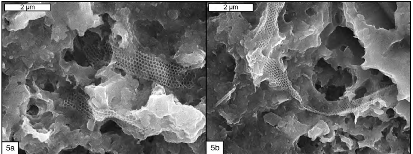
Figure 5. Scanning electron micrographs showing the two different sizes of reticulated filaments with parallel hexagonal chambers. Note the scale is identical in these images. (a) Larger filament. (b) Smaller filament. Hidden Cave pool finger.
