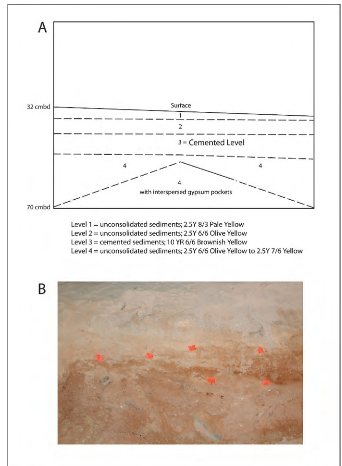
Figure 2. Sedimentary features discussed in text. A. Generalized cross-section from the north wall of excavation square 1N3E indicating overall sedimentary character of deposit. Color changes are noted using descriptions from a Munsell color chart. B. Photograph of the south wall of the excavation showing the cemented level. The top and bottom of the cemented level is bracketed by orange tape.
