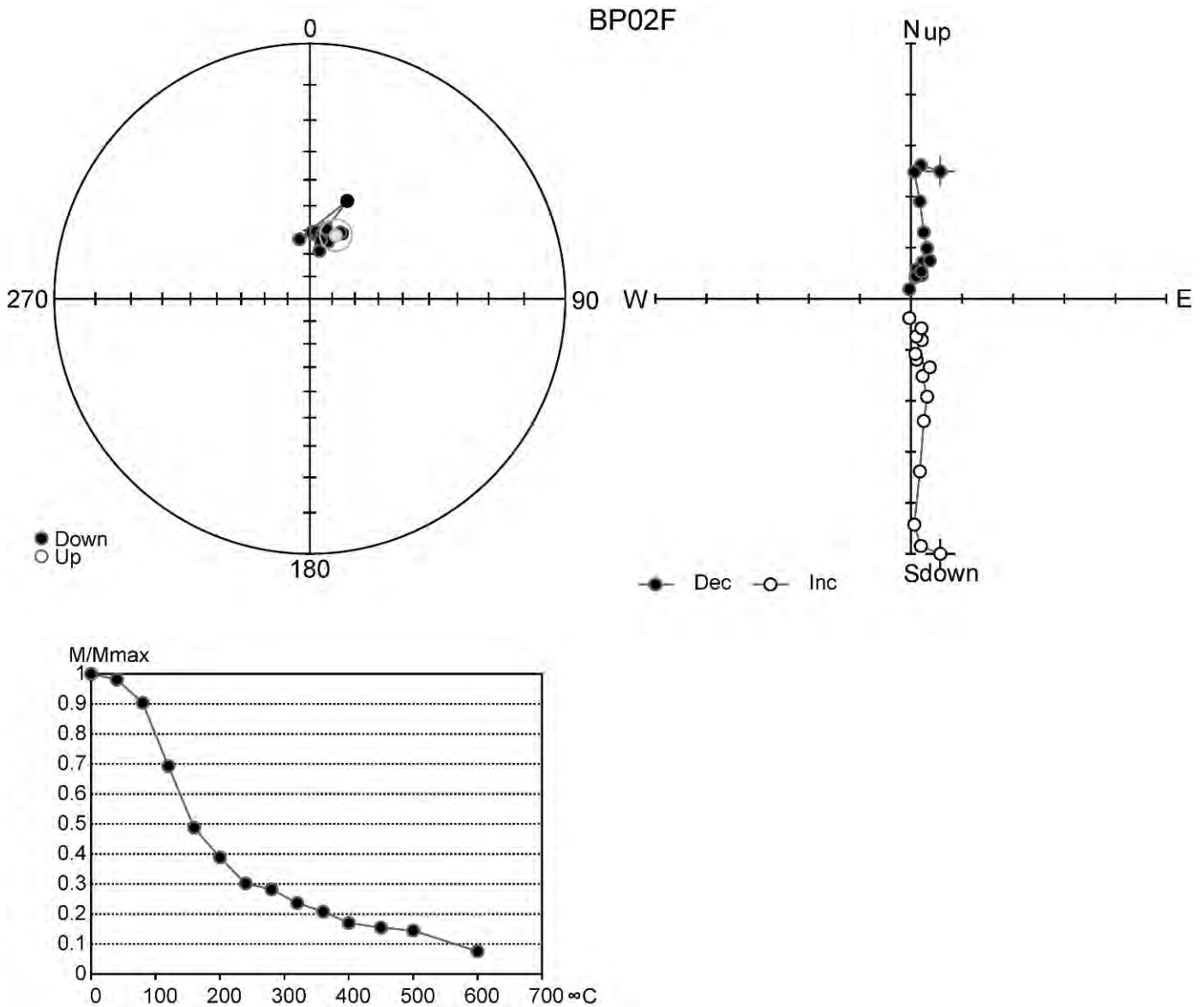
Figure 13. Thermal demagnetization of the flowstone sample BP02F. Top left – directions of magnetization vector during demagnetization process, black circles – projection of vector directions to the lower hemisphere, gray point in the circle – interpreted direction of the primary component of the magnetization vector; top right – Zijderveld diagram, black circles – projection of vector directions into horizontal plane, white circles – projection of vector directions into vertical plane; bottom left – normalized magnetization intensity values during the thermal demagnetization.
