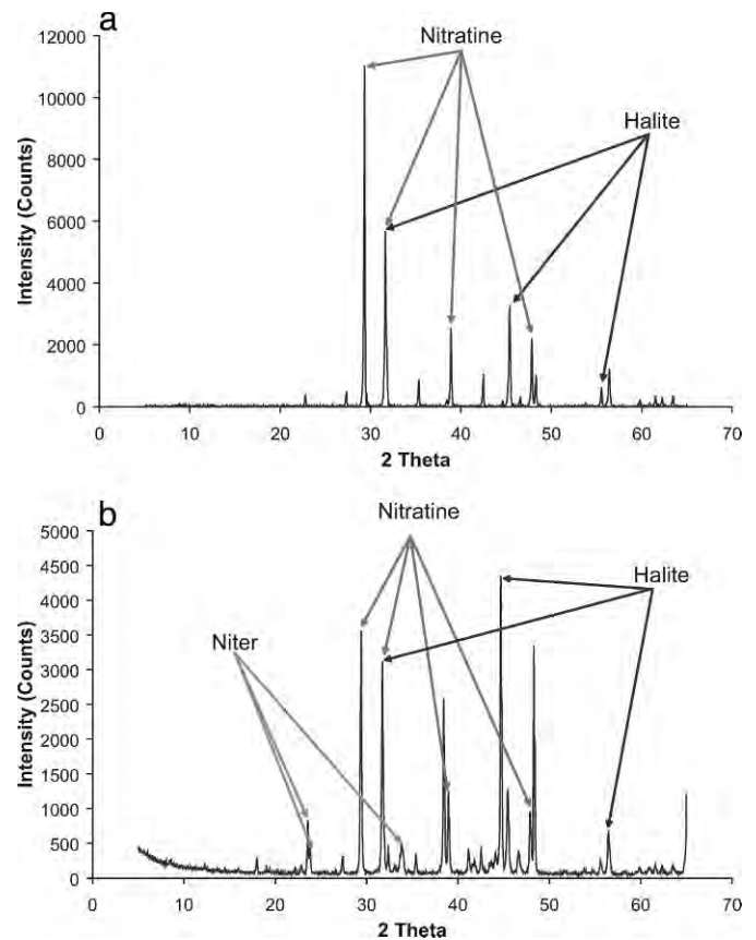
Figure 3. X-ray diffraction (XRD) data. Patterns were generated using Cu K- \alpha radiation. (a) Example of XRD pattern from the cemented level showing the presence of nitratine (peaks marked) (b) XRD pattern of nitratine from the University of Texas collection (peaks marked).
