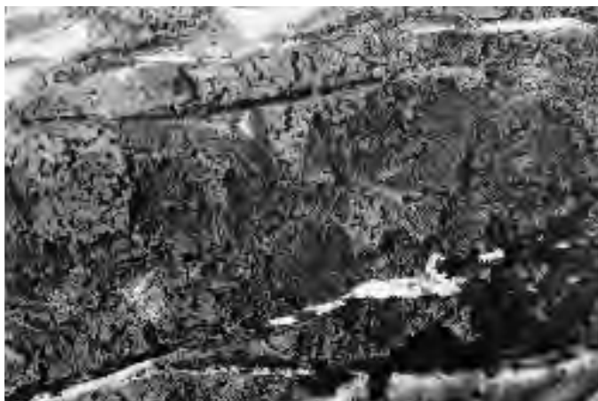
Figure 5. Okher coating on the cave wall, showing visible transformation of small calcite veins into gypsum boxwork.
