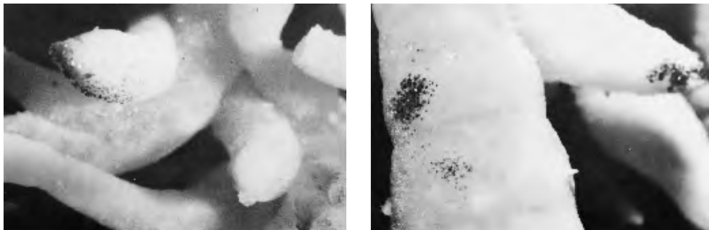
Figure 4. Two views of young secondary fluorite growing upon calcite helictites and gypsum crystals.
