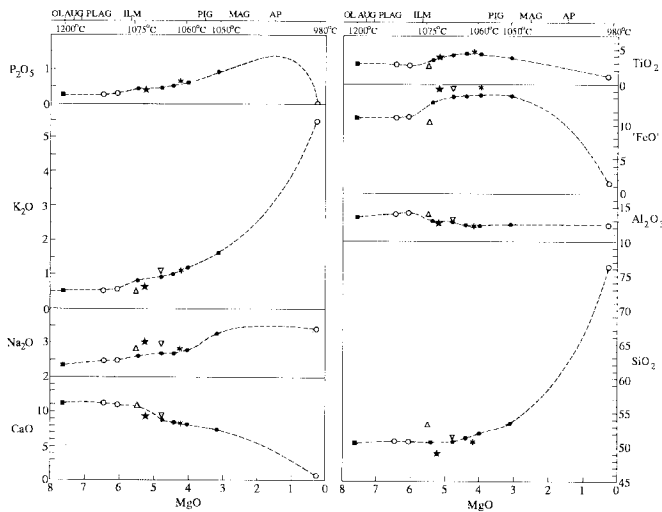
Figure 15. Liquid line of descent, Alae lava lake (Wright & Fiske 1971) with additional plotted lava tube segregations. ■, bulk composition; ○, separated and analyzed glasses; ●, naturally filter pressed oozes; ▲, tubular lava stalactites, (Baird et al. 1985); *, segregation vein sample 68-2-10 (Wright & Okamura, 1977); ▼, tubular lava stalactites (Brigham 1868); ★, HA6 tubular lava stalactites.
