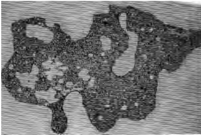
Figure 8. Vuggy fabric in HA2 lining above a small darker tubular lava stalactite. The stalactite is 8 mm long. Photo by M. Palmer.
