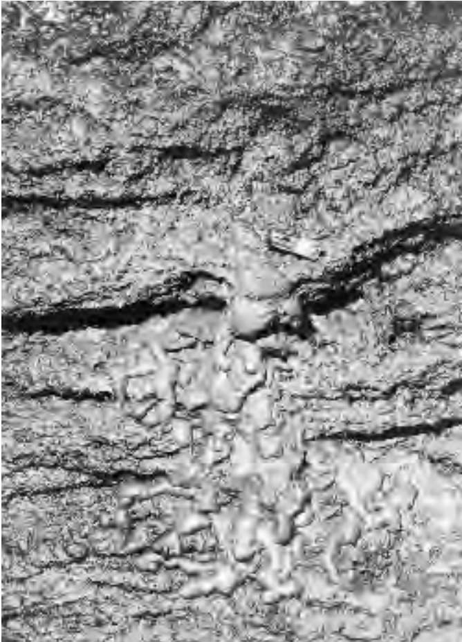
Figure 5 (above). Squeeze-up, Keala Cave. This erupted lava is suspected of being extruded in a similar fashion to tubular lava stalactites. The battery above the rounded cap is 5 cm long. Photo by C. Allred.
