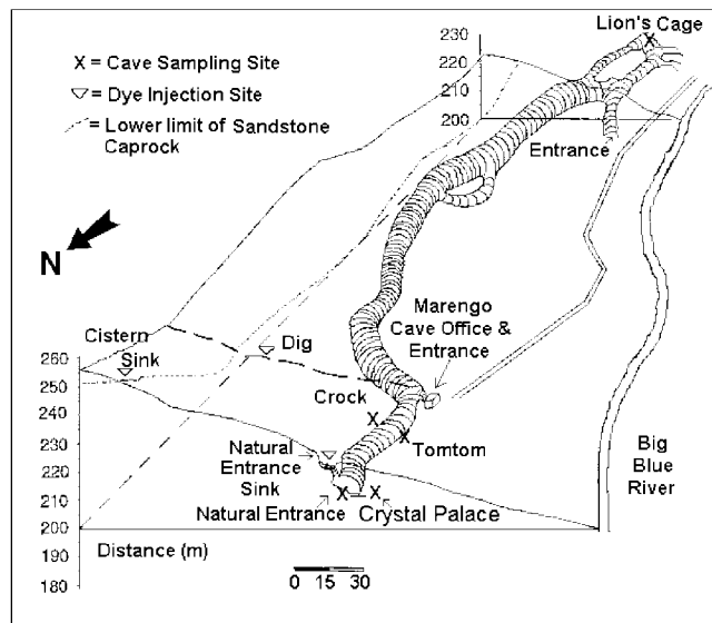
Figure 2. 3-D Model of Upper Marengo Cave, Indiana, a simple low gradient, abandoned river cave. Sites for injection and recovery of dye during the tracer dye tests.
