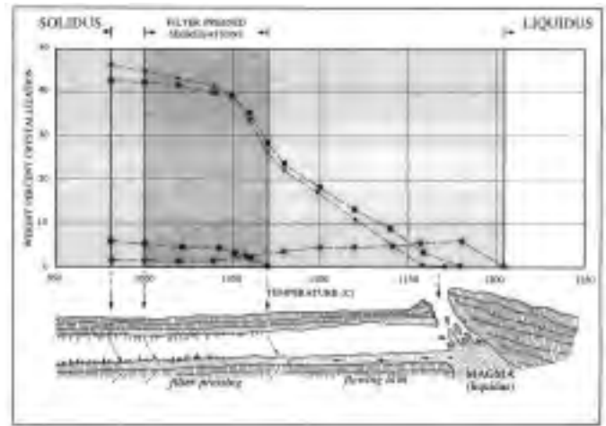
Figure 14. Crystallization of Makaopuhi Lava Lake basalt (data after Wright and Okamura, 1977; Wright and Hiltz, 1987) compared with the inferred solidification and segregation range of a Kilauea lava tube. Approximately 4% of the olivine precipitated at higher temperature is later resorbed. Deflected temperature boundaries through the lava tube are due to a cooler conductive ceiling above the lava river. An eruption temperature of 1165°C was chosen from Swanson (1973). ○, olivine; ■, pyroxene; ▣, plagioclase; ●, Fe-Ti oxides; †, partially crystallized lava.
