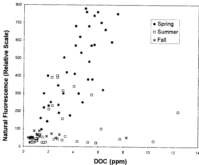
Figure 3. Total Natural Fluorescence vs. Dissolved Organic Carbon (DOC) Concentration (ppm) March - October, 1995 (Divided according to the time of collection).
