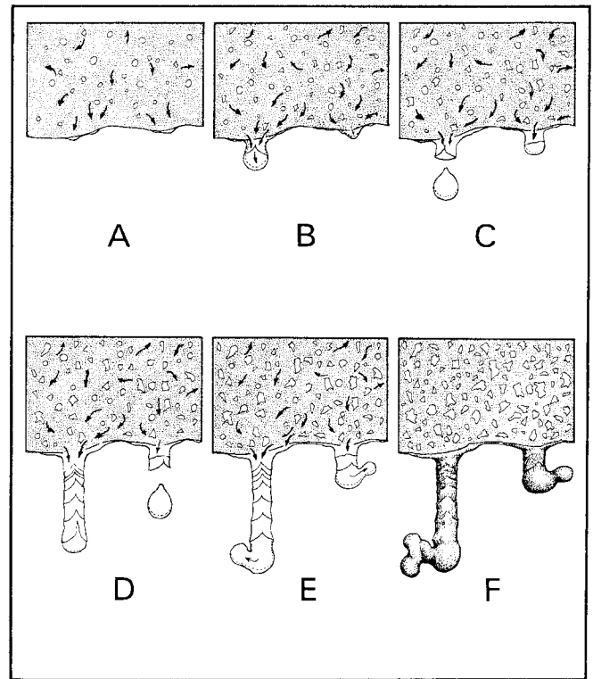
Figure 9. Proposed extrusion of tubular lava stalactites.
