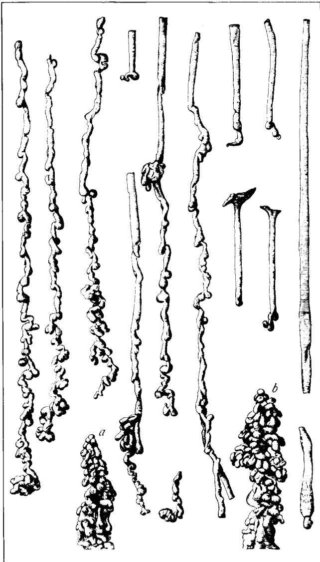
Figure 3. Tubular lava stalactites and lava stalagmites thought to be from Kaumana Cave near Hilo, Hawaii (Dana 1889). The lower ends of the stalactites tend to be more eccentric. As is typical, stalagmites show signs of more fluidity nearer their bottoms.
