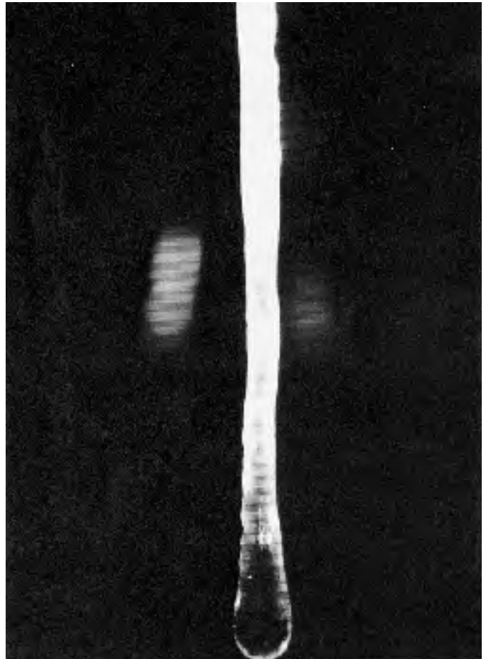
Figure 11. Tubular paraffin stalactite during growth. The stalactite diameter is 3 mm. Photo by C. Allred.
