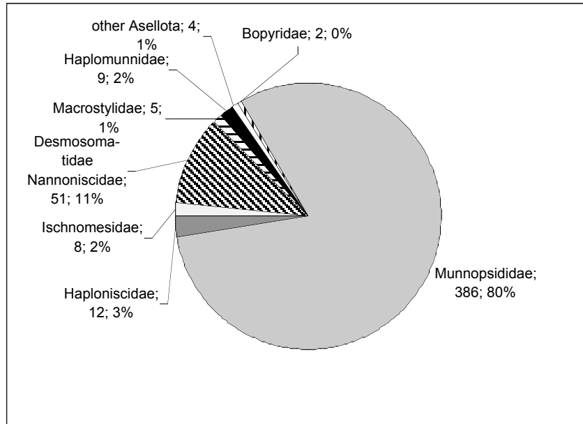
Fig. 9.7: Abundance of isopod families at station 110 in the Weddell Sea
