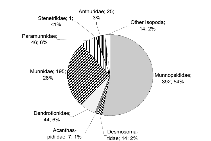
Fig. 9.8: Abundance of isopod families at station 74 off Kapp Norvegia
