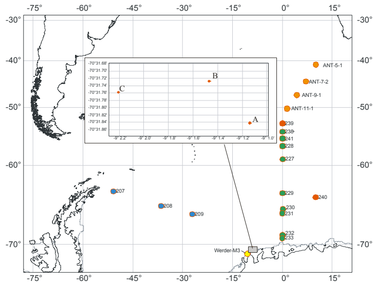
Fig. 4.1: Distribution of moored instruments recovered and deployed during ANT-XXII/3 in the Atlantic sector of the Southern Ocean, along the Greenwich meridian and in the Weddell Sea between Kapp Norvegia and Joinville Island
