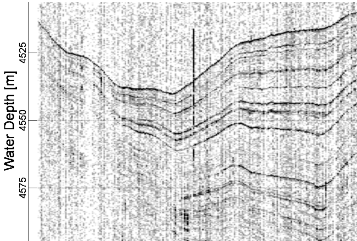
Fig.10.1: Sediment profile at station PS67/21
