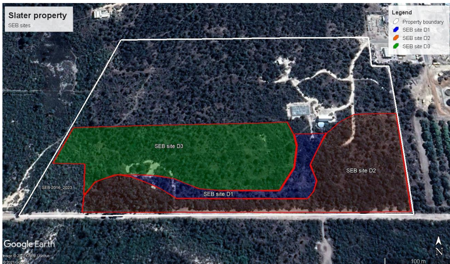
Figure 5. Proposed SEB sites. Site D1 - Very open mallee; Site D2 - Mallee; Site D3 - Low woodland.
