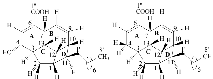
Beilshmiedic acid C (3) Beilshmiedic acid D (4)
