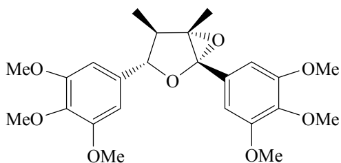
16: 4 \alpha ,5 \alpha -Epoxybeilschmin B
