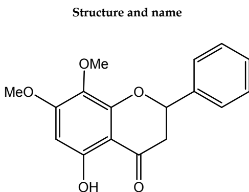
21: 5-Hydroxy-7,8-dimethoxyflavanone
