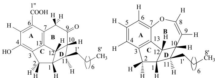
Beilshmiedic acid G (7) Beilshmiedin (8)
