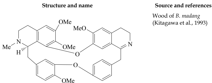
9: Dehatrine
