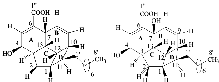
Beilshmiedic acid A (1) Beilshmiedic acid B (2)
