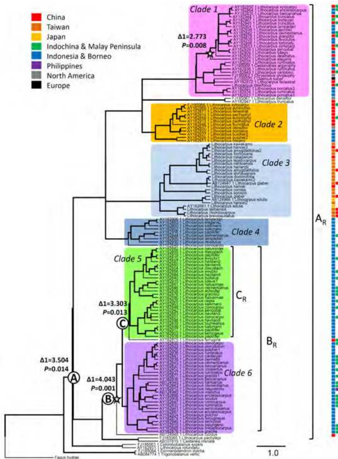
Fig. 1. The Bayesian inference species tree inferred by the Yule’s pure-birth model. The \Delta statistic ( \Delta 1 ) and its tail probability are indicated in the nodes of the significant diversification rate shift (A~C). The nodes marked by the stars are significantly shifted in the diversification rate that was estimated in the gene tree. Clades A R , B R and C R are the derived clades with high diversification rates of nodes A, B, and C, respectively, namely radiation clades. Six major clades of Lithocarpus (Clades 1~6) are indicated in colored blocks. The colored boxes to the right indicate the distribution area of the species. The bold lines represent branches with >90% statistical support by posterior probability.
