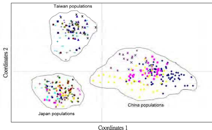
Fig. 5. Distribution of varieties in a two-dimensional PCoA space based on the ISSR data in Toxicodendron radicans spp. hispidum and spp. orientale . According to the ISSR result, the three groups were separated by three different regions, including Japan, Taiwan, and China.
