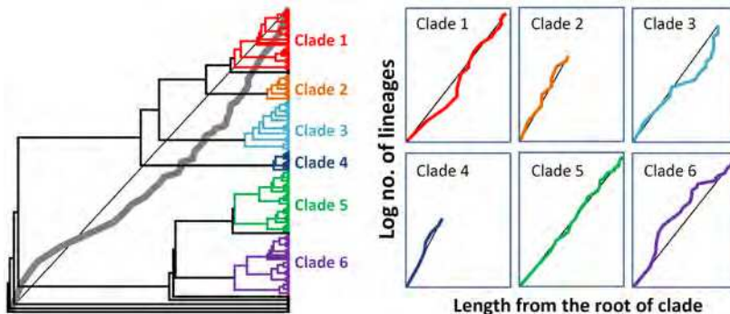
Fig. 2. Plot of the lineage-through-time (LTT) analysis of Lithocarpus using the species tree inferred by the Bayesian-based Yule's pure birth model. The left panel is the speciation tree inferred by Yule's pure-birth model, and the gray curve indicates the LTT curve (scaled by the log of the number of lineages). The right panel is the LTT curves of the specific clades (Clade 1~6, indicated in different colors). Straight lines under the LTT curves indicate the averaged LTT in constant growth rate.
