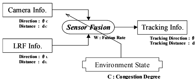
Fig. 15. Rate-Changeable Environmental Adaptive Sensor Fusion Model
