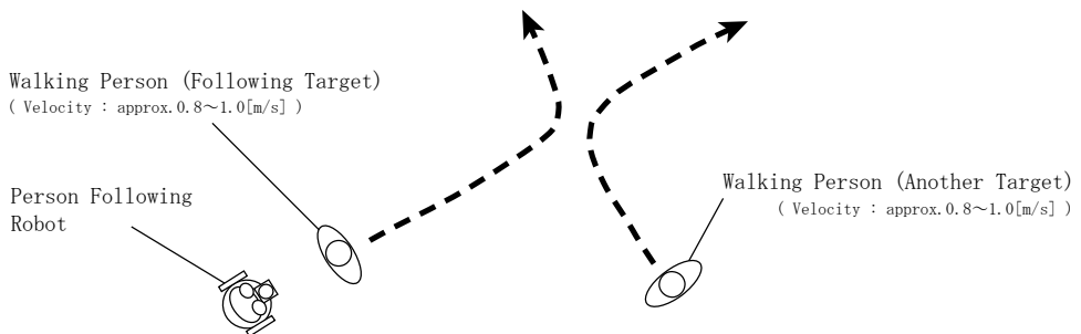
Fig. 21. Experimental Situation: Pseudo Crossing Motion (Two People Walking Meet and Part)
