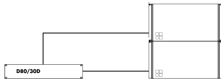
D80/30D amplifier in 2-Way Active mode for J-SUB and/or J-INFRA
