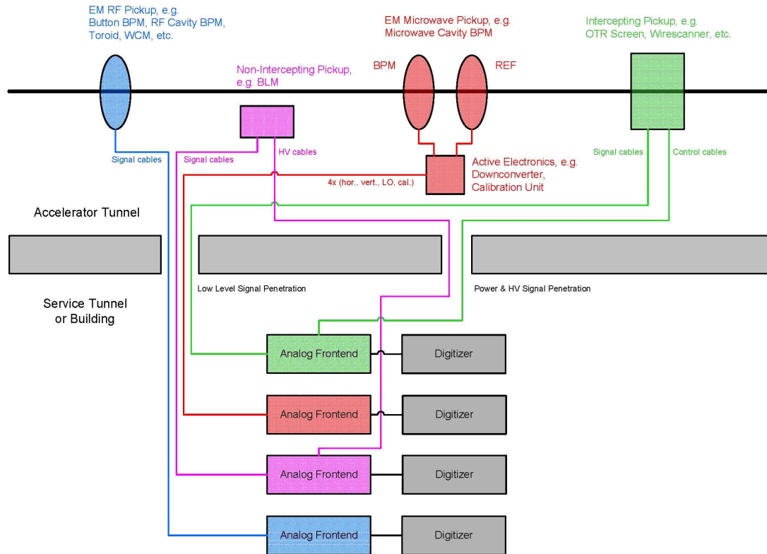
FIGURE 3.10-3. Generalised Schematic of Beam Pickups and Read-Out Systems.
