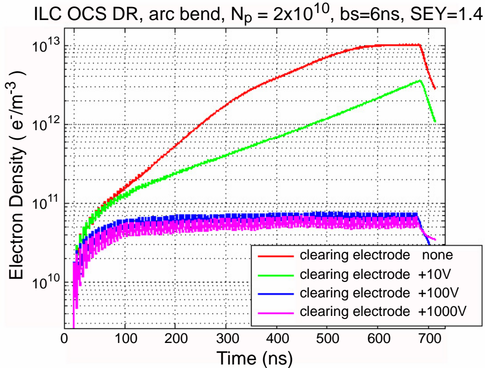
FIGURE 2.4-6. Electron cloud buildup in an arc bend of the 6.7 km ring and suppression effect of clearing electrodes biased at the indicated voltages.
