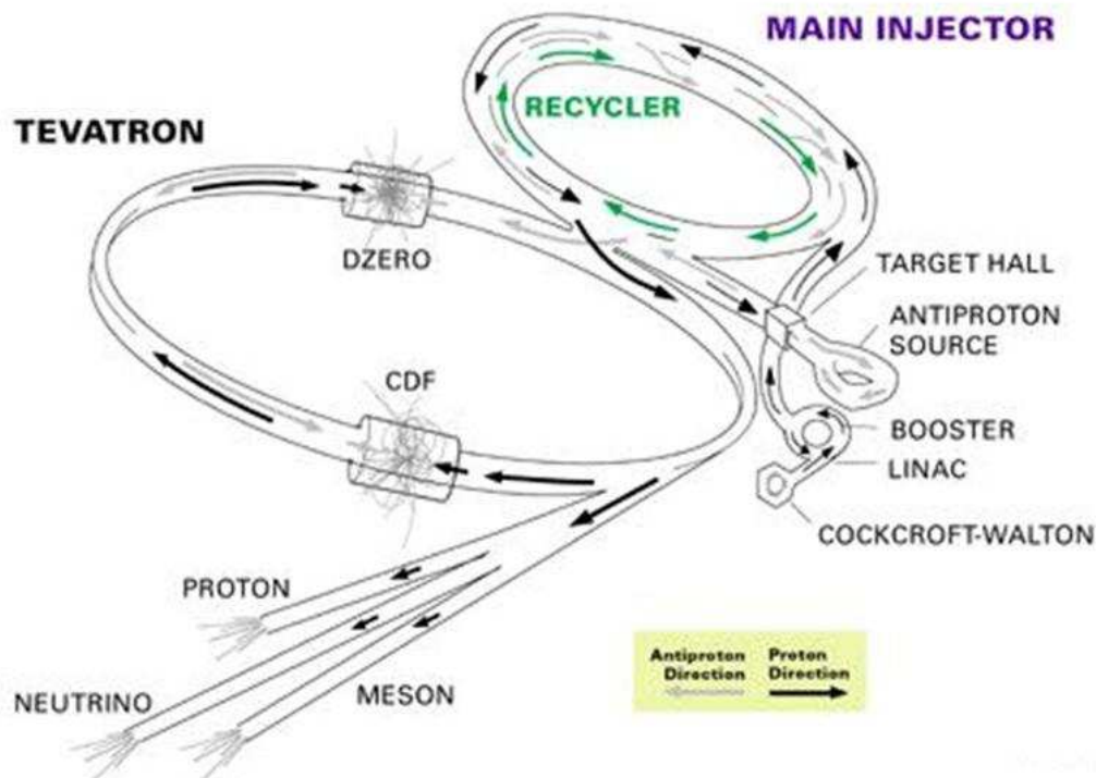
Figure 2.1.1: Schematic view of the accelerator chain at Fermilab.
