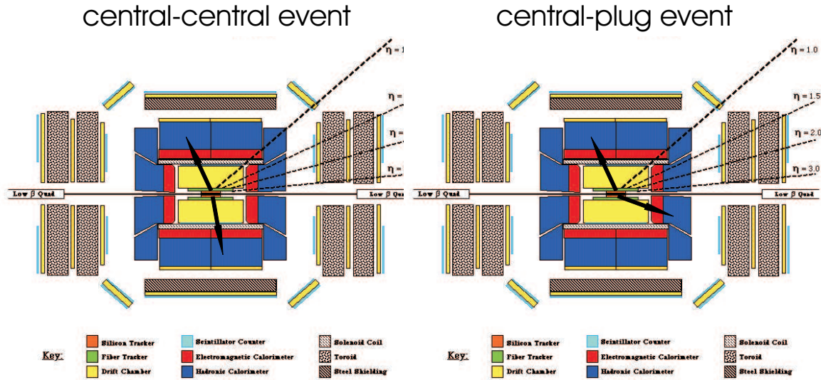
Figure 5.2.1: A schematic view of the two different event types. On the left a Z boson event with both electrons central, on the right a Z boson event with only one electron detected in the central calorimeter and the other one in the plug calorimeter. The electrons are indicated by the black arrows.
