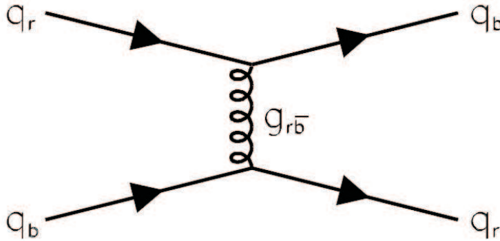
Figure 1.3.2: An example of quark-quark scattering by the exchange of a gluon. The colors are indicated.
