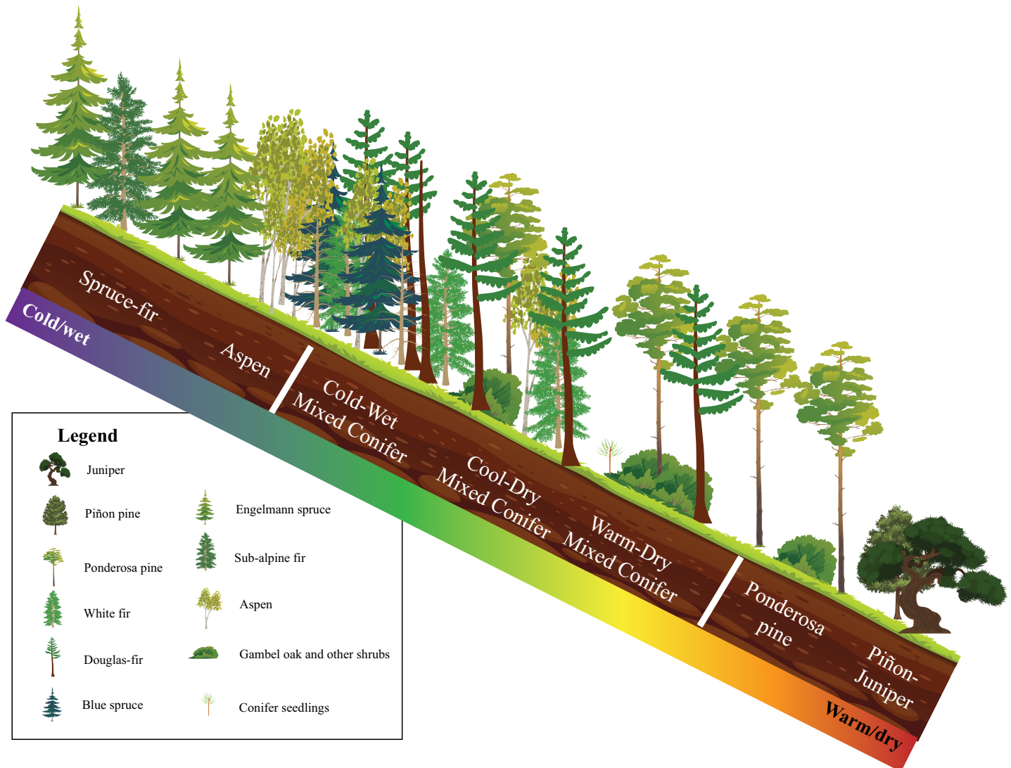
Figure 2: Graphical representation of forest types in the San Juan Mountain region represented on a hillslope where the lowest elevations are the warmest /driest sites and higher elevations are the coldest/wettest. Forest types not discussed in detail in this knowledge synthesis, such as pinon-juniper are still depicted for reference.
