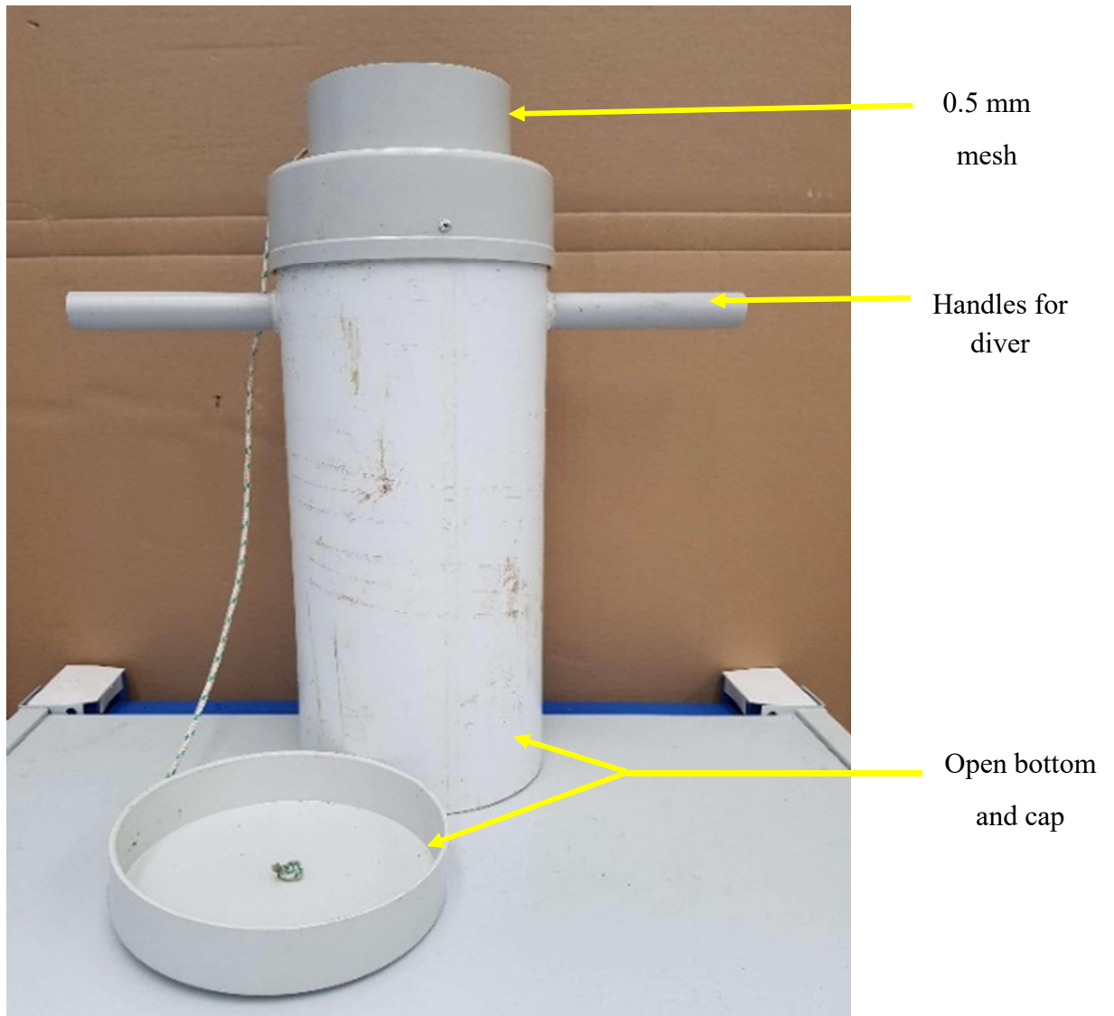
Appendix B. PVC sampling corer design. Photograph illustrates the 0.5 mm mesh top of the cylinder, the handles the diver uses to push the corer into the bryozoan or sediment, and open bottom cap that is used to seal the container.
