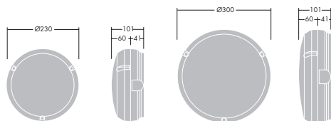
Small round, black base + opal diffuser
