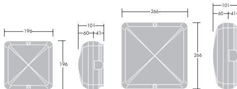
Small square, black base + opal diffuser
