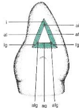
Fig. 6-20 Schematic representation (for descriptive purpose) of Fig. 6-18 illustrating tooth preparation line angles and point angles. Line angles are axiolingual (al), linguogingival (lg), axiogingival (ag), faciogingival (fg), axiofacial (af), and incisal (i). Point angles are axiolinguogingival (algl), axiofaciogingival (afgl), and axioincisal (ai). (Note that names for incisal line angle and point angle are exceptions to the general naming rule.)
