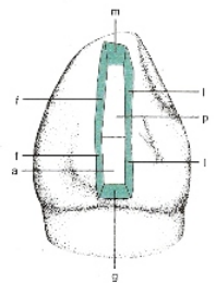
Fig. 6-22 Schematic representation (for descriptive purpose) of Fig. 6-21 illustrating tooth preparation walls: facial (f) of proximal and incisal portions, gingival (g), lingual (l) of proximal and incisal portions, axial (a), and mesial (m).
