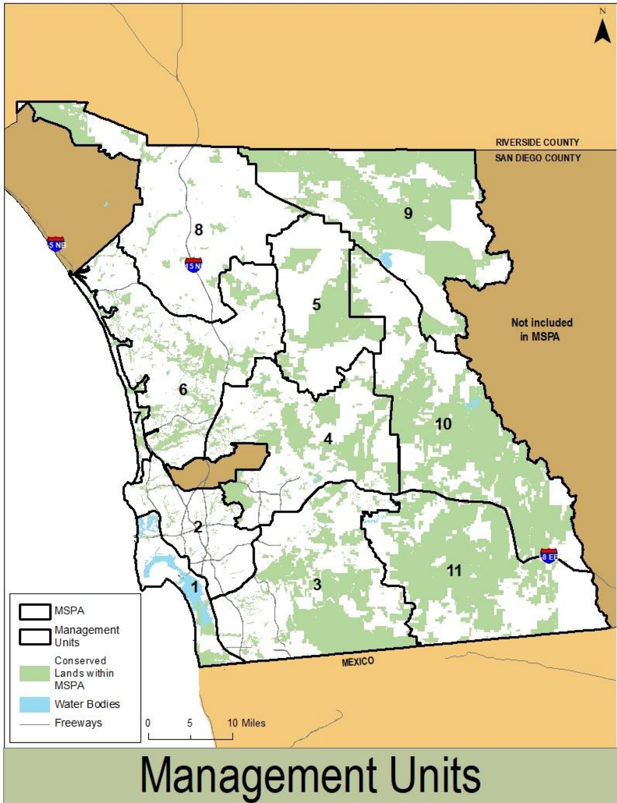
Figure 2. Management Units (MUs) within the MSPA.
