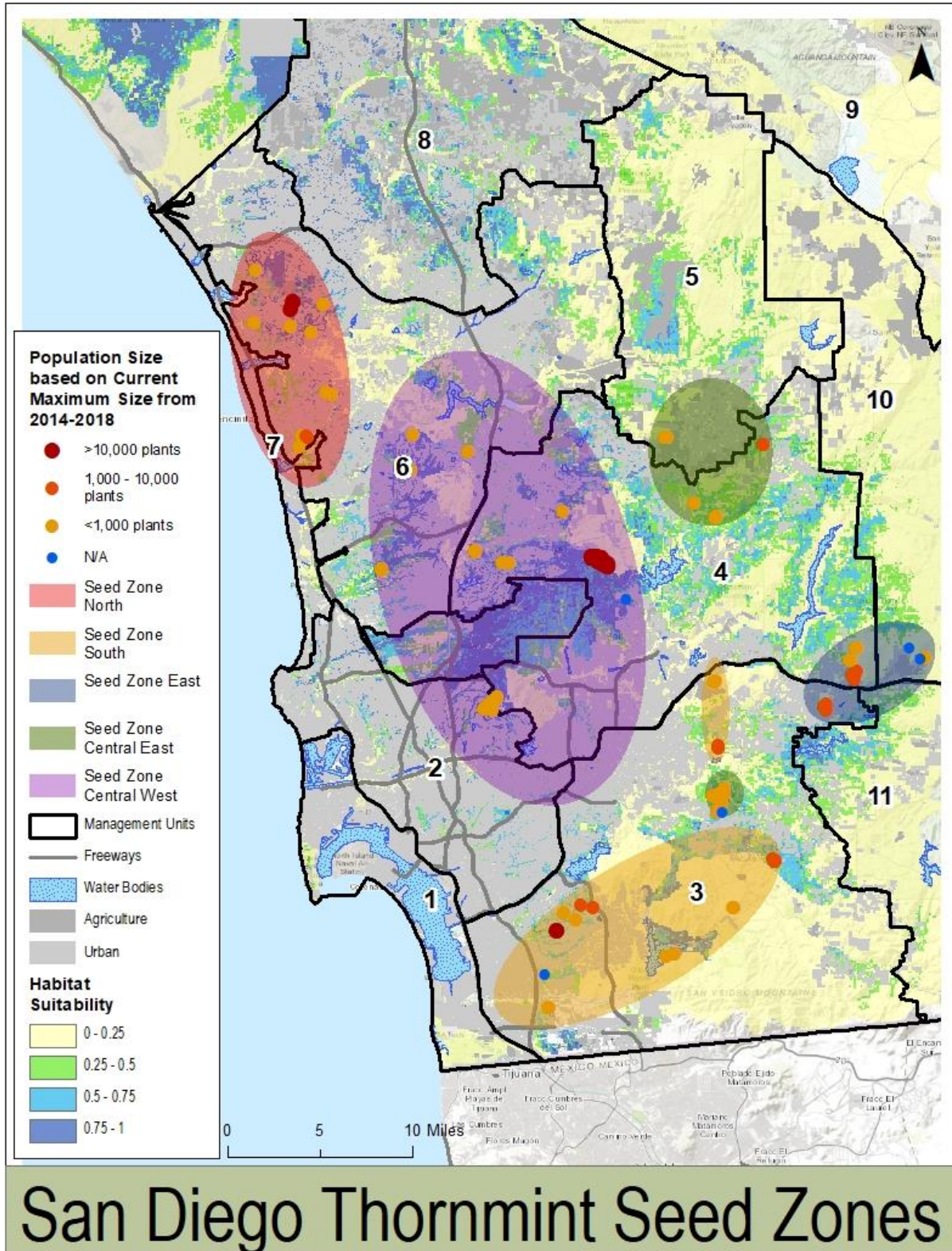
Figure 11. San Diego Thornmint: Seed Zones.
