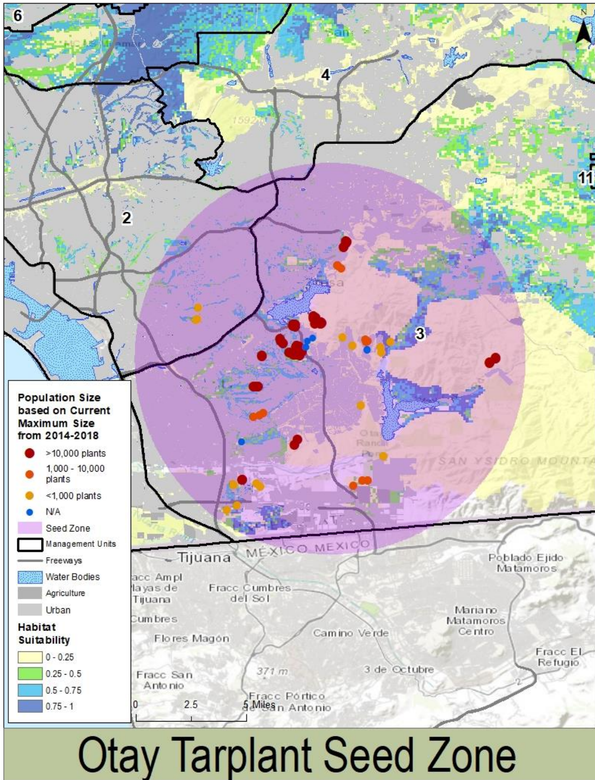
Figure 19. Otay Tarplant: Seed Zone.
