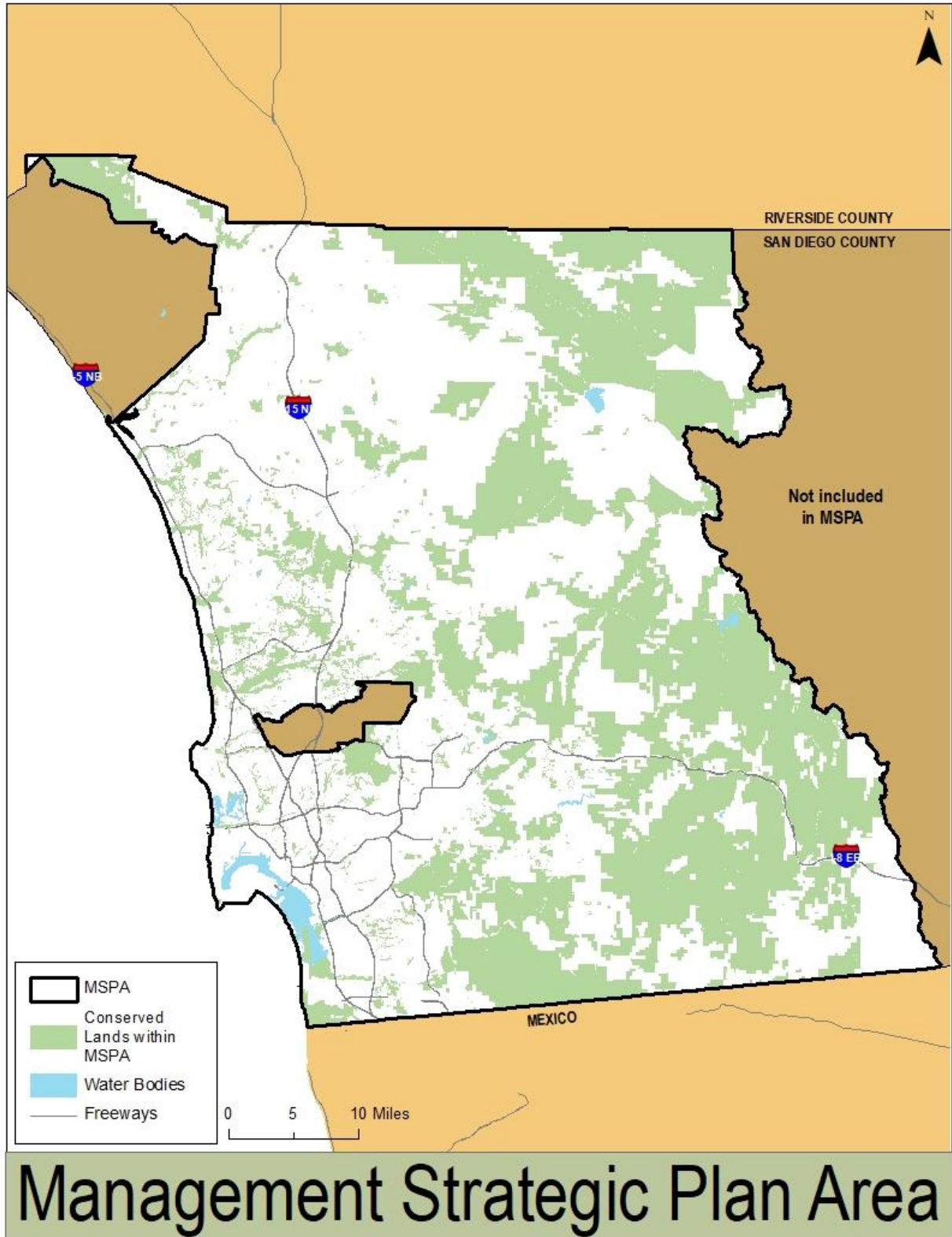
Figure 1. MSP Roadmap Area (MSPA) in Western San Diego County.
