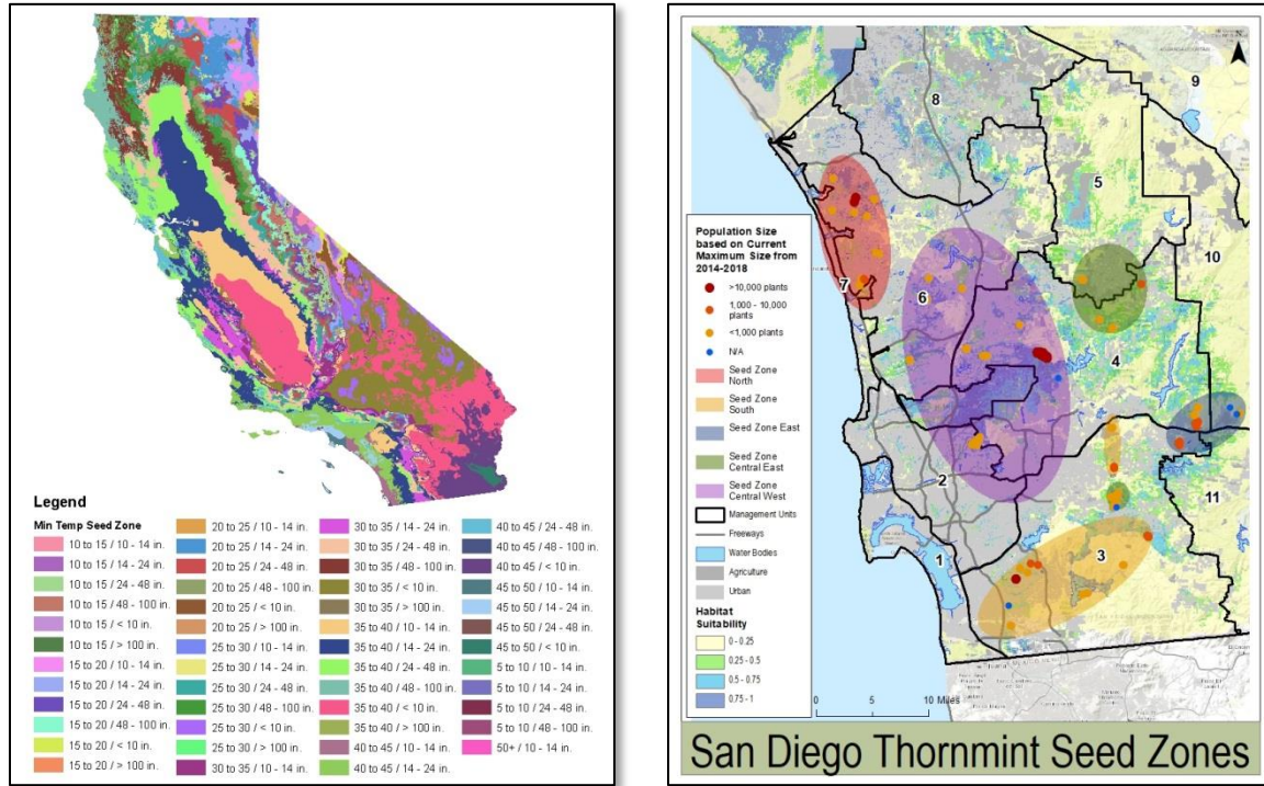
Figure 4. Seed Zone Maps: (left) Provisional Seed Zones for California Native Plants based on Temperature and Precipitation ( http://www.forestseedlingnetwork.com ), (right) Genetic Seed Zones for San Diego Thornmint in San Diego County.
