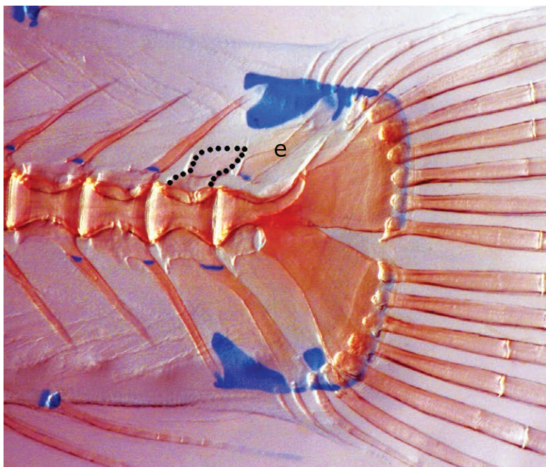
Figure 2. Emblemariopsis signifer , caudal osteology: black dots=truncated neural spine; e=epural last vertebra; blue=cartilage (B. Victor).
