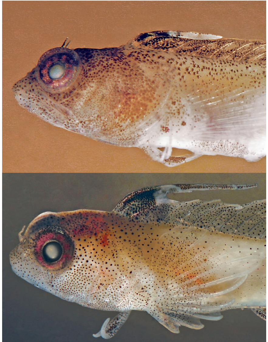
Figure 53. Comparison of length of first dorsal-fin spines in preserved TP E. occidentalis , ANSP 192008 (upper) and E. carib , holotype, UF 179454 (lower) (Benjamin Victor).
