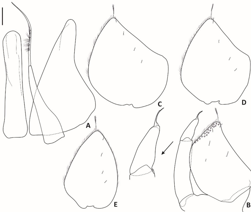
FIGURE 8. Alponiscus (Illyrionethes) lossinii n. sp. Paratype male CBSSC IT2379 from Medvjeda špilja. A, genital papilla and pleopod 1; B, pleopod 2 with enlargement of endopod tip; C, pleopod 3 exopod; D, pleopod 4 exopod; E, pleopod 5 exopod. Scale bar: 0.1 mm.
