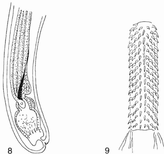
Figures 8 and 9 (8) Tubular cement glands and posterior end of Filisoma . (9) Proboscis of Paratenuisentis ambiguus .
