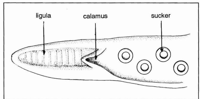
Figure 9 Hectocotylized arm of an octopod.
