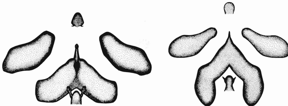
Figure 18 Anal palps, funnel organs, and funnel valves. Rossia palpebroso (left); Rossia megaptera (right).
