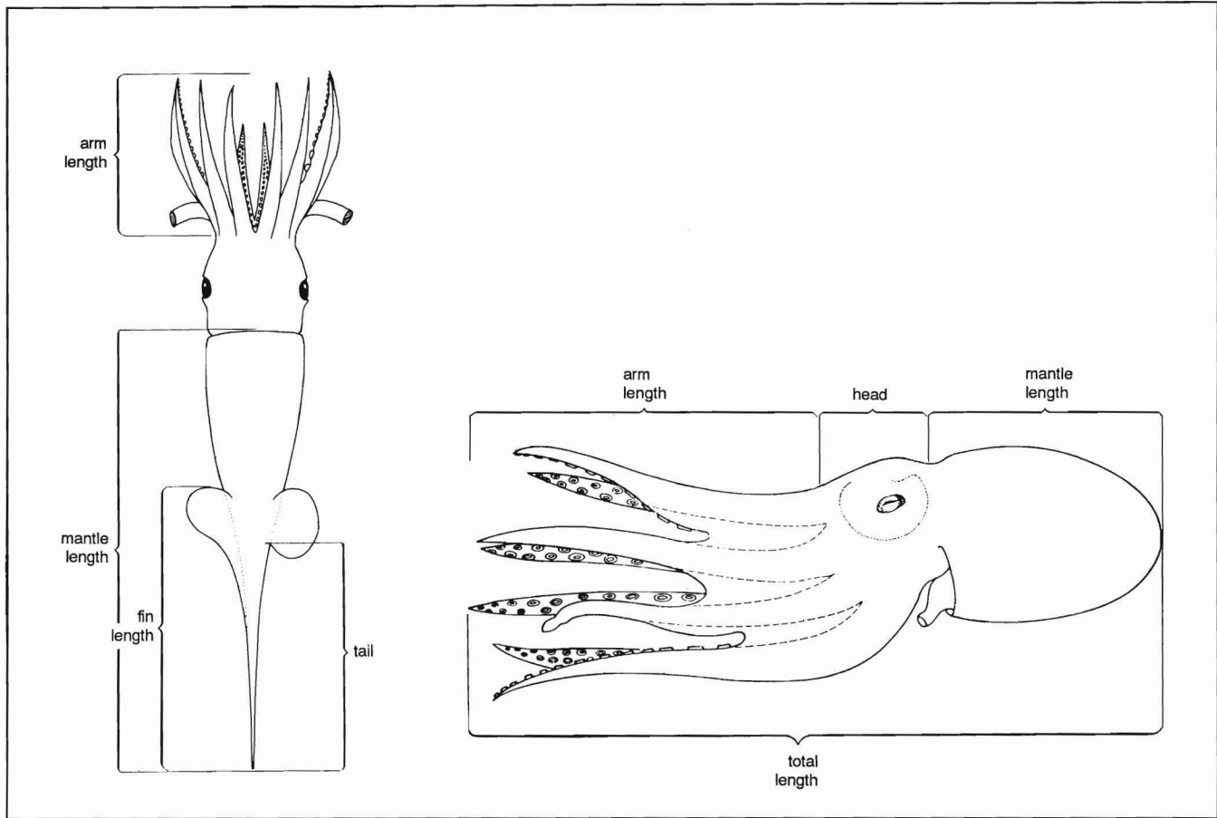
Figure 10 Some standard measurements on cephalopods. Squid (left); octopus (right).
