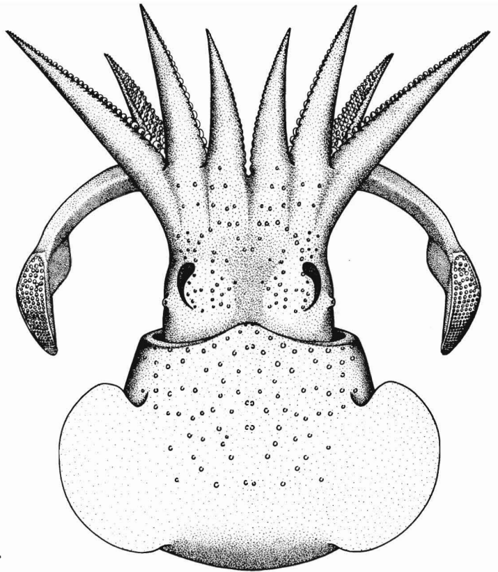
Figure 19 Rossia palpebrosa (dorsal aspect).
