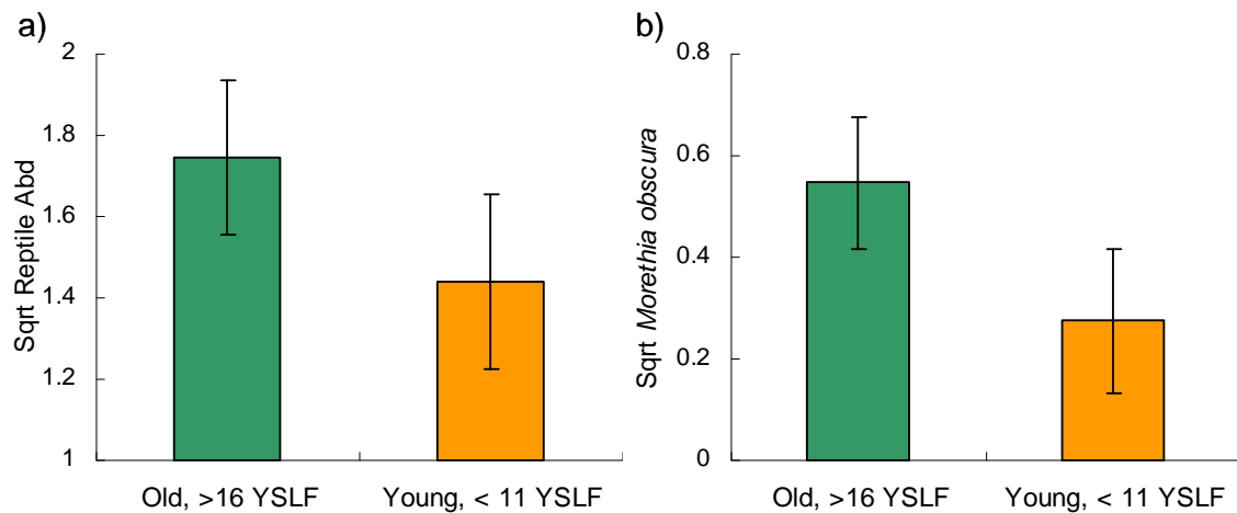
Figure 7.1: Significant differences in the mean ( \pm 95%CI) of a) reptile abundance and b) abundance of M. obscura between long unburnt (Old) and recently burnt (Young) sites.
