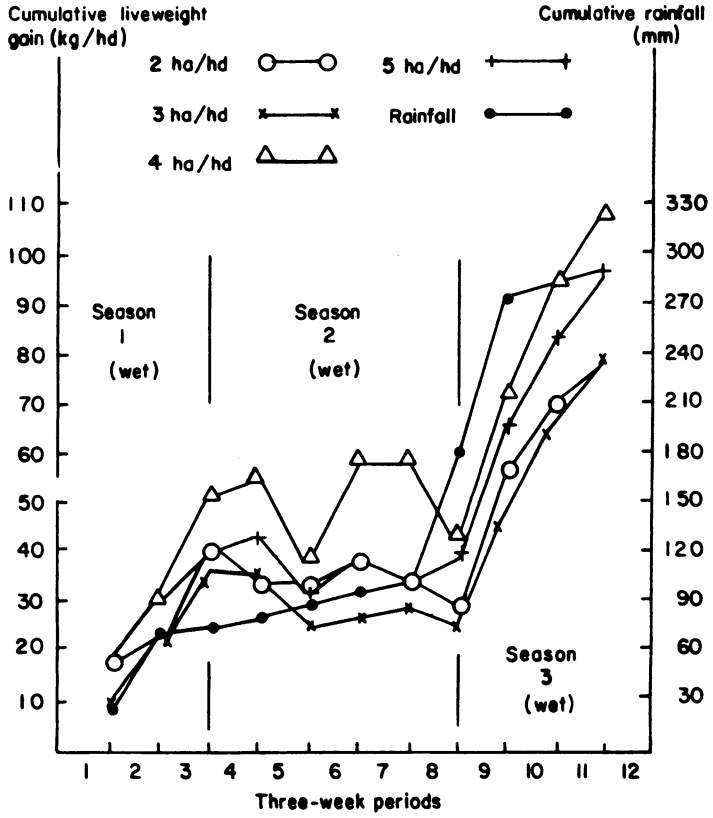
Figure 1. Liveweight gain/rainfall, animal series 1 (3.6.74-20.1.75).
