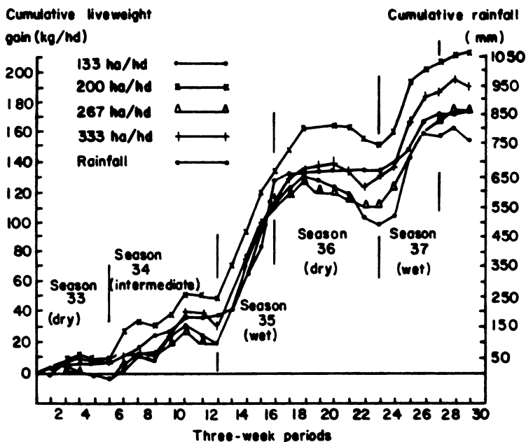
Figure 8. Liveweight gain/rainfall, animal series (9.7.85-30.3.87).
