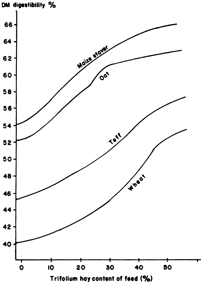
Figure 1. Effect of addition of Trifolium hay on dry-matter digestibility of cereal straws.
