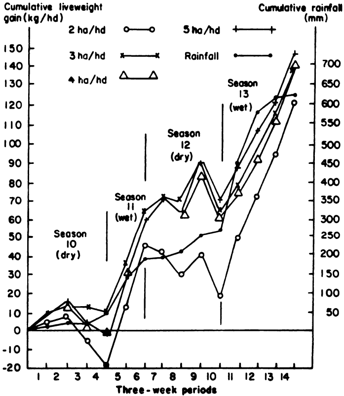
Figure 3. Liveweight gain/rainfall, animal series 3 (20.7.77-11.9.77).
