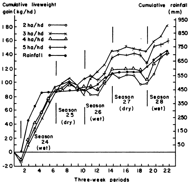
Figure 6. Liveweight gain/rainfall, animal series (16.3.81-21.6.82).
