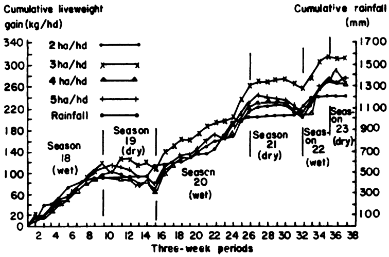
Figure 5. Liveweight gain/rainfall, animal series (11.1.79-22.3.81).
