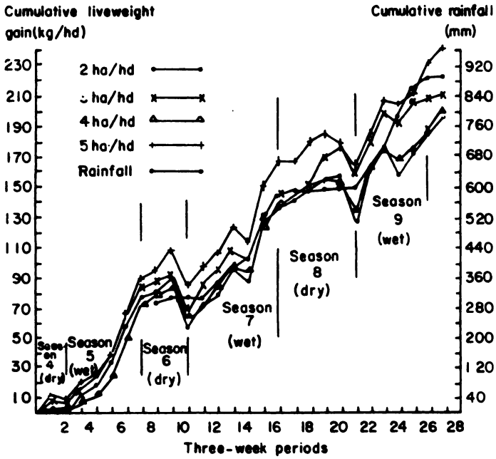
Figure 2. Liveweight gain/rainfall, animal series 2 (17.2.75-30.8.76).
