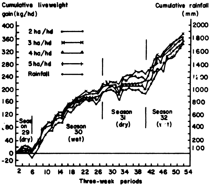
Figure 7. Liveweight gain/rainfall, animal series (12.7.82-23.7.85).
