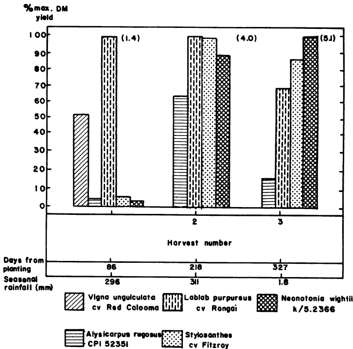
Figure 1a. Relative dry-matter yield (expressed as a percentage of the maximum dry-matter yield) for five legume swards grown at Maruba, Kenya. Swards were planted on 30-10-85 and the third harvest was taken 327 days later on 22-9-86. Absolute dry-matter yield in tonnes ha -1 is shown in parentheses for each harvest.
