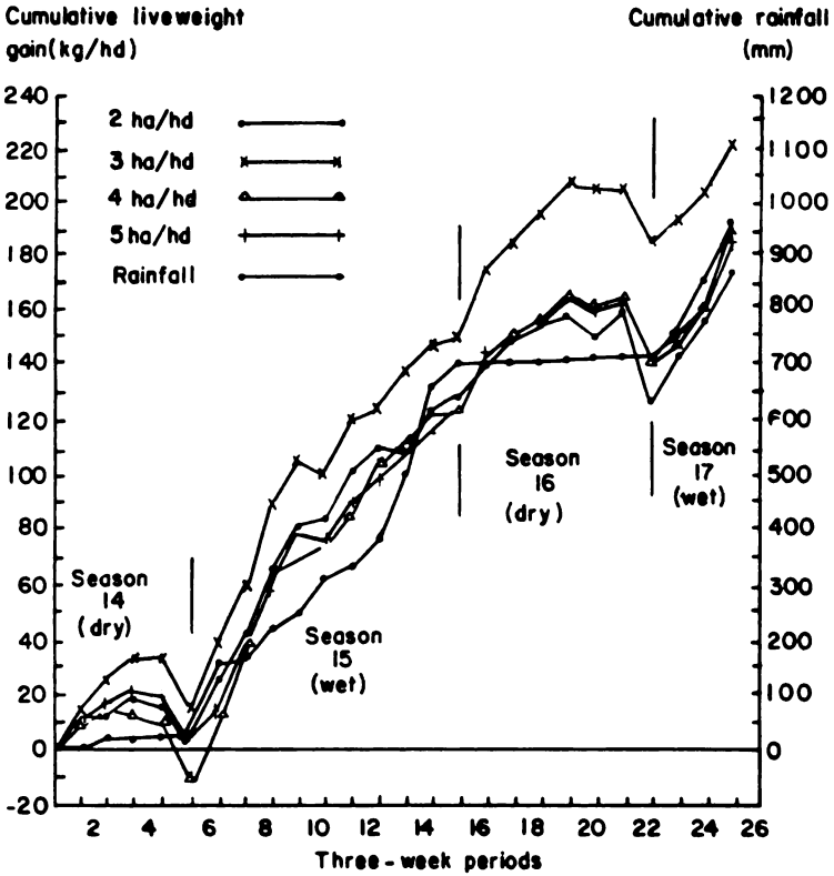
Figure 4. Liveweight gain/rainfall, animal series 4 (1.8.77-8.1.79).
