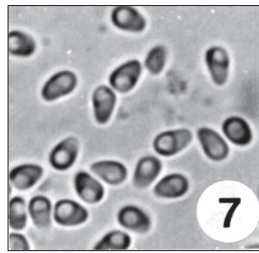
Fig. 7. Fresh spores of Microsporidium sp2 in Selene dorsalis ( \times 2000 )
