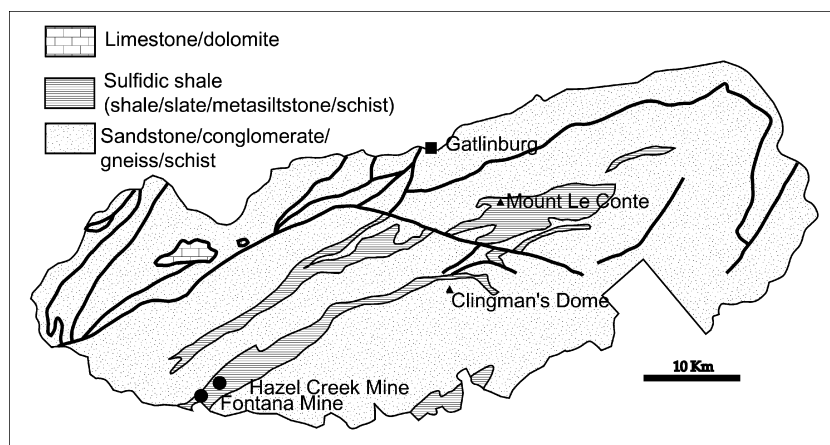
Fig. 2 Lithochemical map of Great Smoky Mountains National Park showing the distribution of various rock types. Heavy lines are faults. Modified from Southworth (1995)
