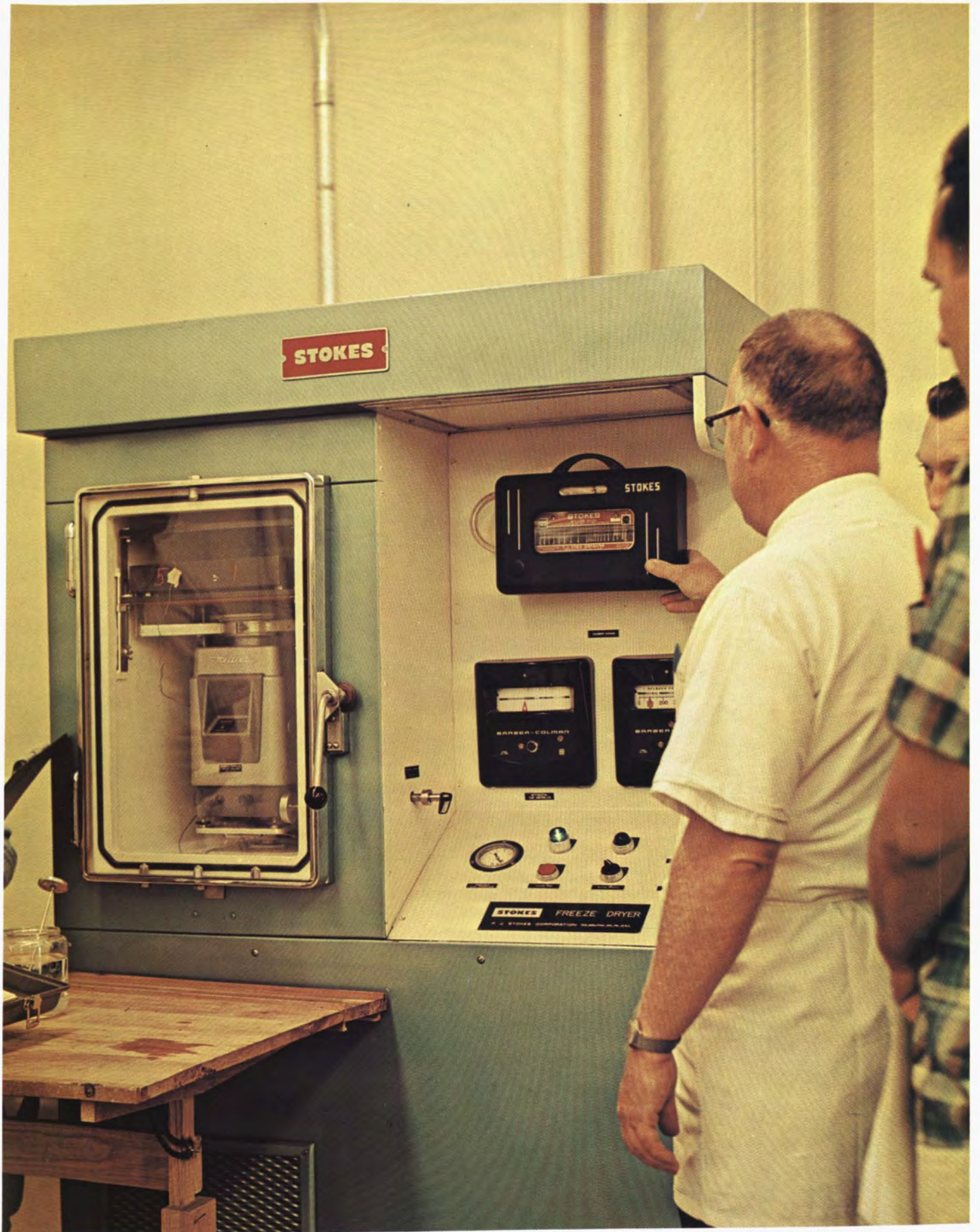
The Stokes freeze dryer uses the sublimation process to remove ice crystals from frozen foods under high vacuum to produce high quality dehydrated foods for campers and homemakers.
