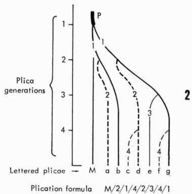
FIG. 4. Diagrammatic construction of plication patterns in Neospirifer dunbari showing mode of distinguishing successive plica generations and recording them as plication formulas. 1. Fold. 2. Sulcus. [Explanation: P. denotes primary plica extending from beak to first bifurcation; M denotes mid-line unbranched plica which originates independently of primary or other plicae.]
