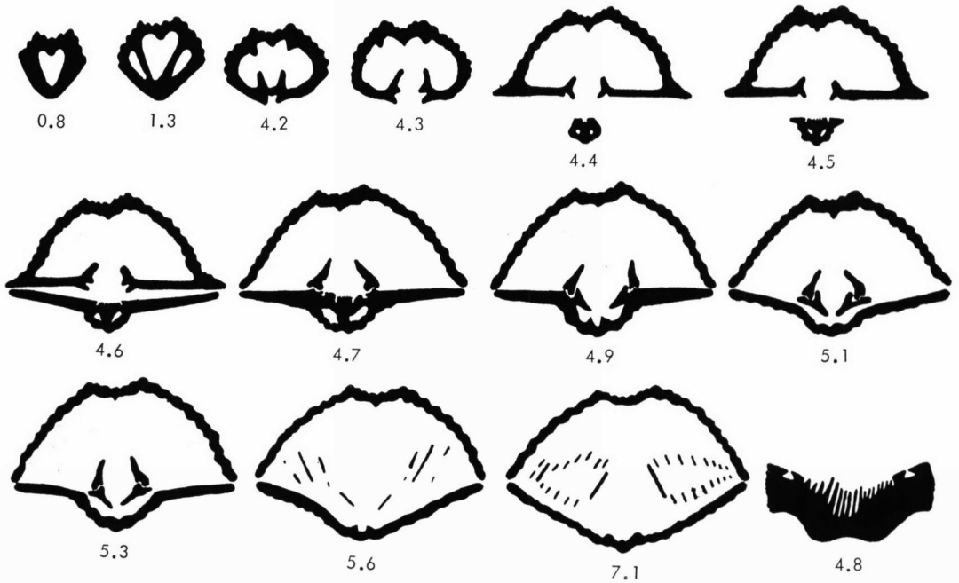
FIG. 10. Serial transverse sections of Spirifer rockymontanus MARCOU. The first section (upper left) is near the beak of the pedicle valve and succeeding sections are progressively farther from the beak, the precise distance being indicated in millimeters beneath each section; all illustrations are oriented with pedicle valve above and brachial valve below; all are \times 3 , except the last (lower right) which shows the cardinal process, \times 15 .
