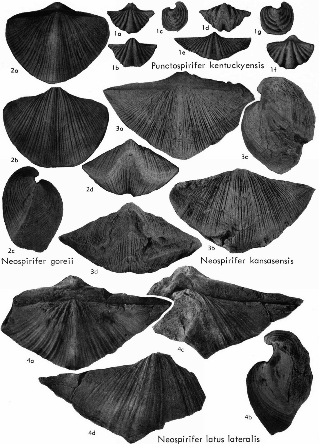
FIG. 7. Species of Punctospirifer and Neospirifer (see facing page for explanation).
