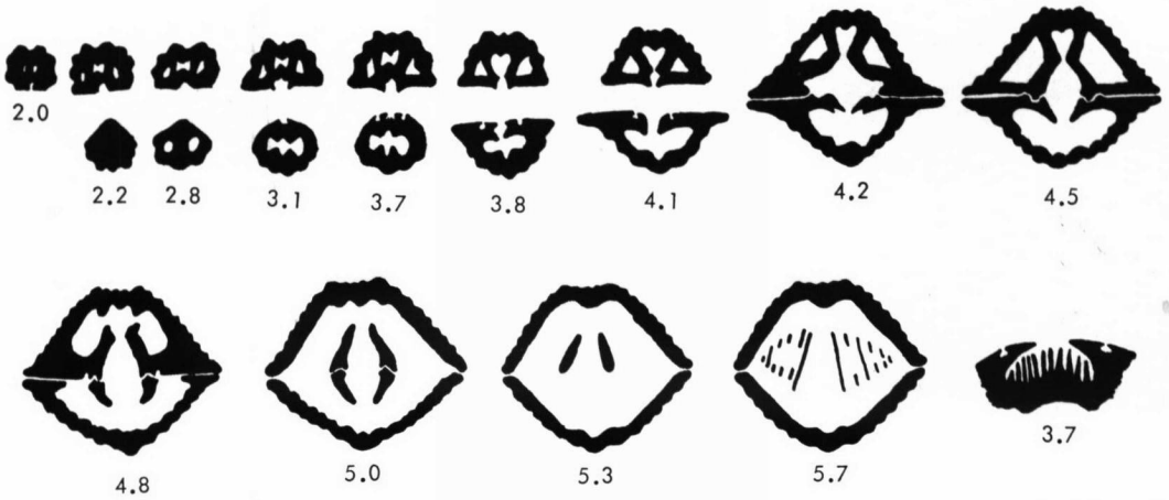
FIG. 11. Serial transverse sections of Spirifer opimus HALL. The first section (upper left) is near the beak of the pedicle valve and succeeding sections are progressively farther from the beak, the precise distance being indicated in millimeters beneath each section; all illustrations are oriented with pedicle valve above and brachial valve below; all are \times 3 , except the last (lower right) which shows cardinal process, \times 15 .
