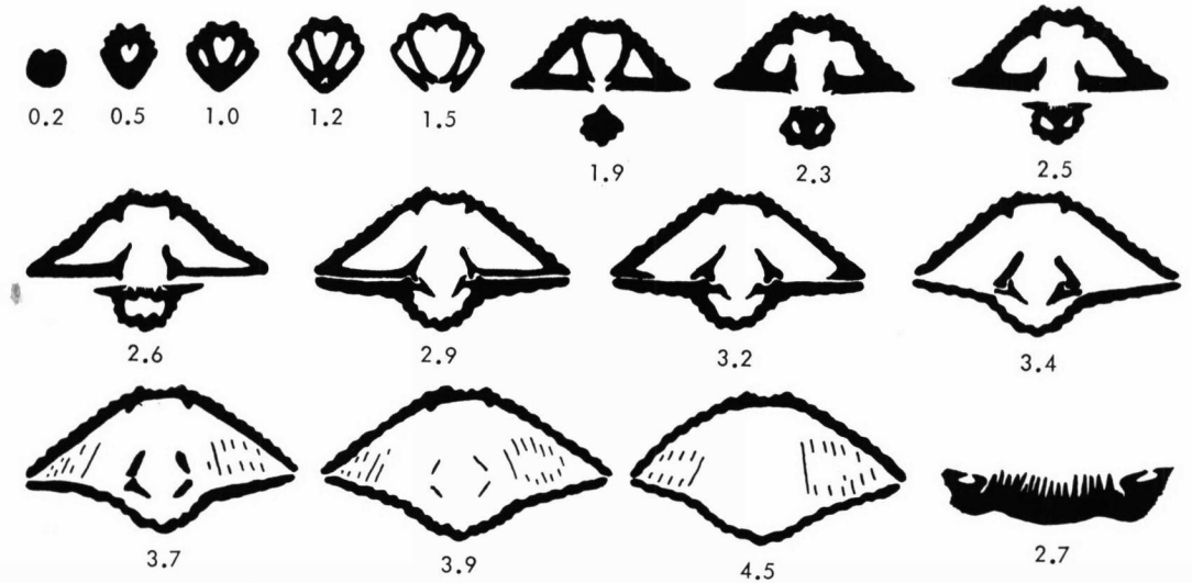
FIG. 12. Serial transverse sections of Spirifer occiduus SADLICK. The first section (upper left) is near the beak of the pedicle valve and succeeding sections are progressively farther from the beak, the precise distance being indicated in millimeters beneath each section; all illustrations are oriented with pedicle valve above and brachial valve below; all are \times 3 , except the last (lower right) which shows cardinal process, \times 15 .
