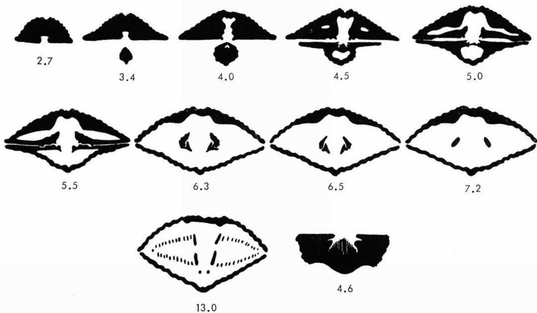
FIG. 22. Serial transverse sections of Neospirifer goreii MATHER. The first section (upper left) is near the beak of the pedicle valve and succeeding sections are progressively farther from the beak, the precise distance being indicated in millimeters beneath each section; all illustrations are oriented with pedicle valve above and brachial below; all are \times 1.5 , except the last (lower right) which shows cardinal process, \times 15 .
