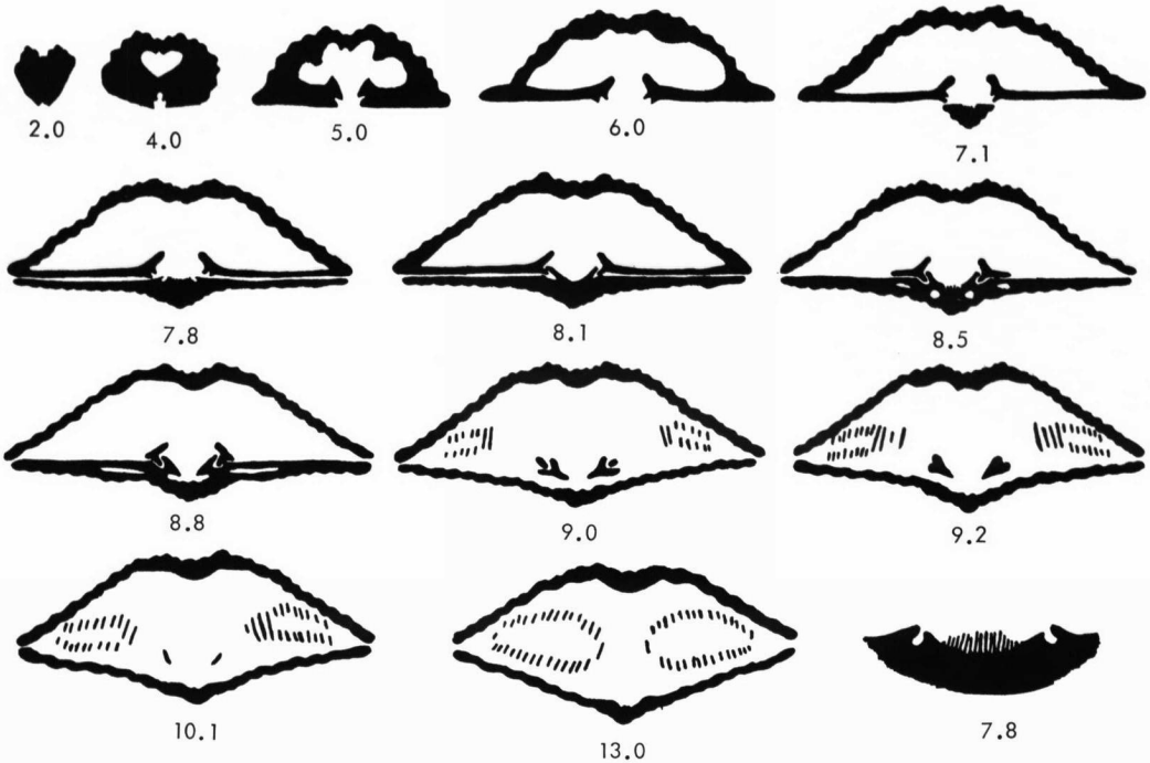
FIG. 14. Serial transverse sections of Neospirifer dunbari dunbari KING. The first section (upper left) is near the beak of the pedicle valve and succeeding sections are progressively farther from the beak, the precise distance being indicated in millimeters beneath each section; all illustrations are oriented with pedicle valve above and brachial valve below; all are \times 1.5 , except the last (lower right) which shows cardinal process, \times 8 .
