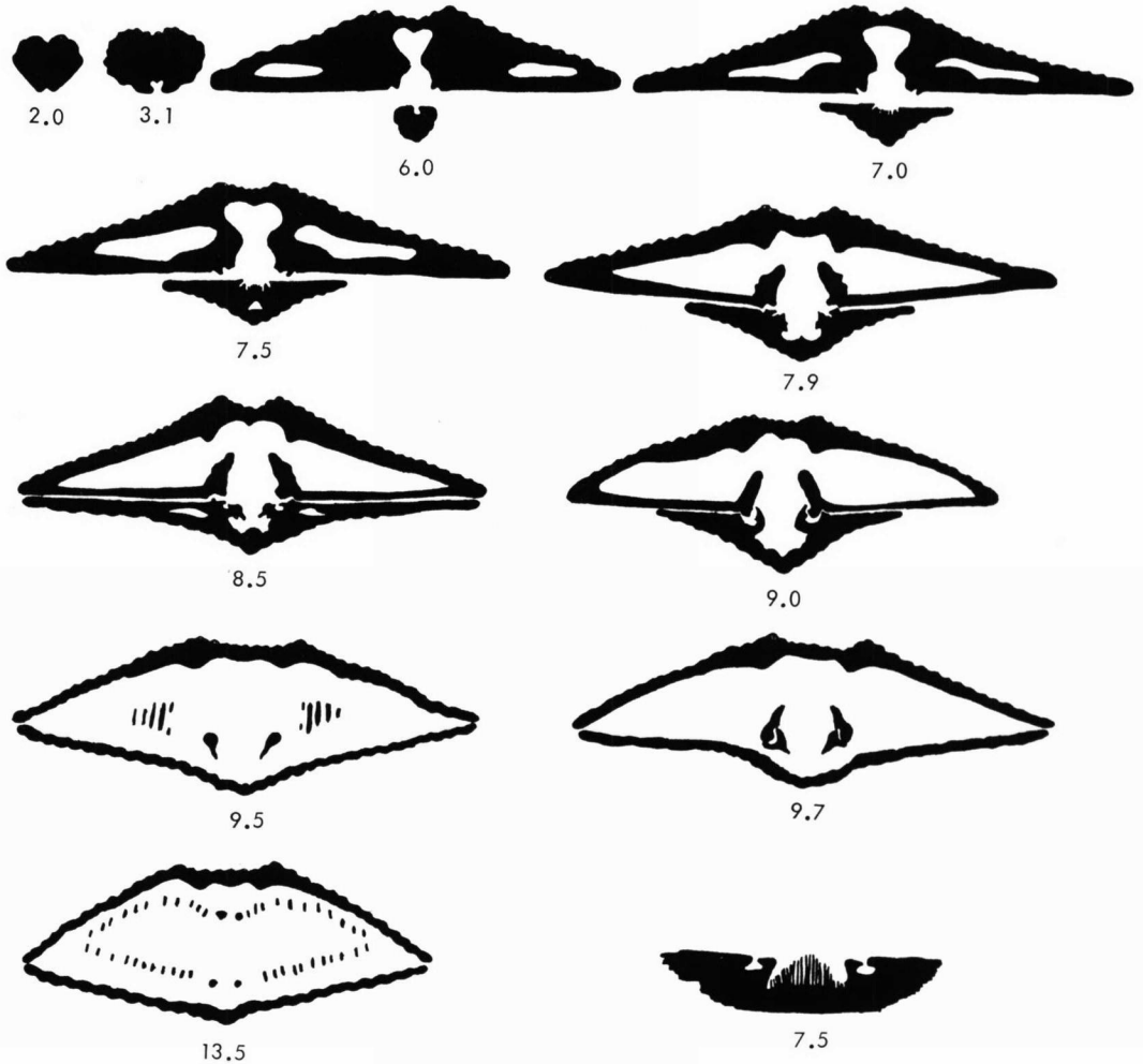
FIG. 20. Serial transverse sections of Neospirifer kansasensis SWALLOW. The first section (upper left) is near the beak of the pedicle valve and succeeding sections are progressively farther from the beak, the precise distance being indicated in millimeters beneath each section; all illustrations are oriented with pedicle valve above and brachial valve below; all are \times 1.5 , except the last (lower right) which shows cardinal process, \times 15 .
