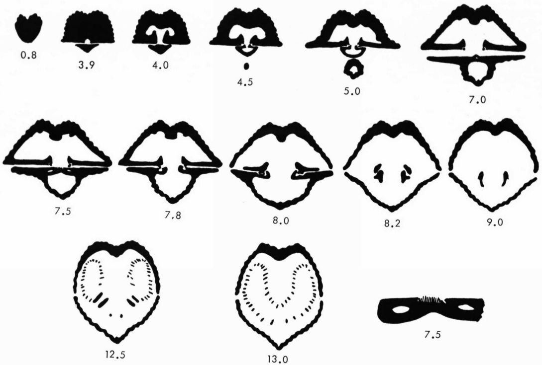
FIG. 21. Serial transverse sections of Neospirifer texanus MEEK. The first section (upper left) is near the beak of the pedicle valve and succeeding sections are progressively farther from the beak, the precise distance being indicated in millimeters beneath each section; all illustrations are oriented with pedicle valve above and brachial valve below; all are \times 1.5 , except the last (lower left) which shows cardinal process, \times 15 .
