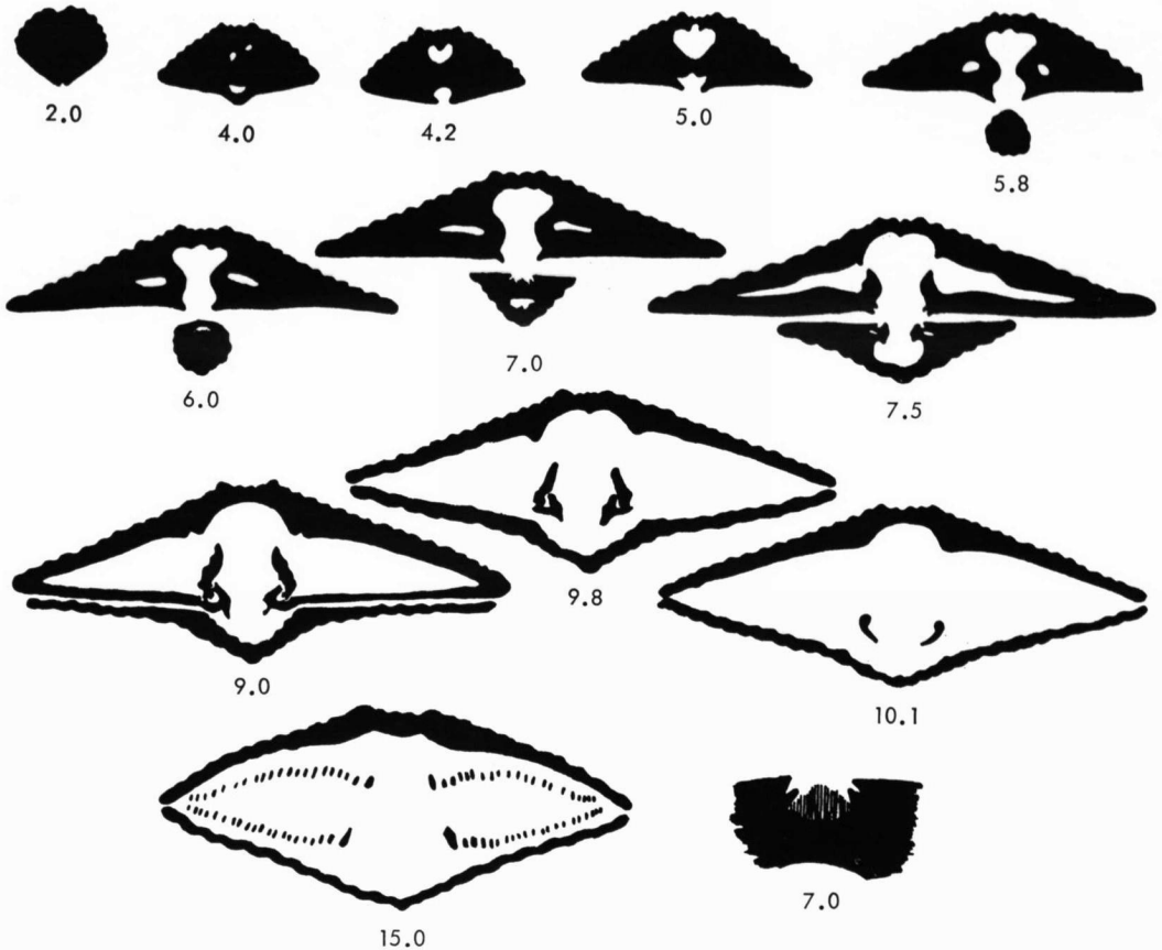
FIG. 17. Serial transverse sections of Neospirifer cameratus MORTON. The first section (upper left) is near the beak of the pedicle valve and succeeding sections are progressively farther from the beak, the precise distance being indicated in millimeters beneath each section; all illustrations are oriented with pedicle valve above and brachial valve below; all are \times 1.5 , except the last (lower right) which shows cardinal process, \times 8 .
