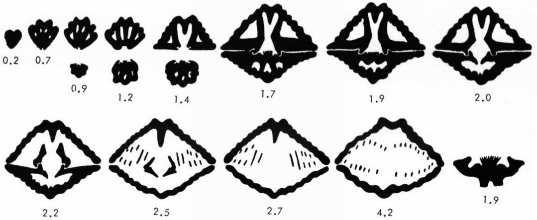
FIG. 8. Serial transverse sections of Punctospirifer kentuckyensis SHUMARD. The first section (upper left) is near the beak of the pedicle valve and succeeding sections are progressively farther from the beak, the precise distance being indicated in millimeters beneath each section; all illustrations are oriented with pedicle valve above and brachial valve below; all are \times 3 , except the last (lower right) which shows cardinal process, \times 15 .
