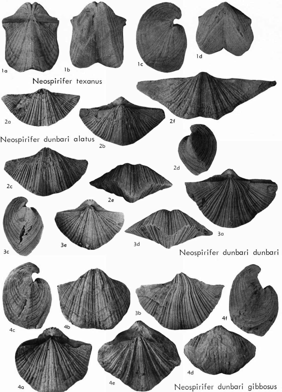
FIG. 13. Species and subspecies of Neospirifer (see facing page for explanation).
