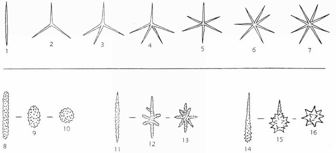
FIG. 1. Meristic variation in euasters s.s. (1-7) contrasted with passages from monaxon to pseudoeuaster (8-16).
