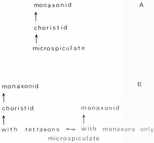
FIG. 9. Relationship of microscopiculate, choristid, and monaxonid sponges, as inferred by DENDY (A) and REID (B). Under DENDY's picture of phylogeny (1905, 1916, 1921), all monaxonid sponges must be forms derived from choristids. According to REID's different picture, monaxonids may be forms derived either from choristids, or from sponges with no spicules but monaxons before the evolution of megascleres. The latter mode of origin is thought probable for the Desmacidontida (compare also REID, 1963, fig. 2: Sigmatosclerophora=Desmacidontida).
