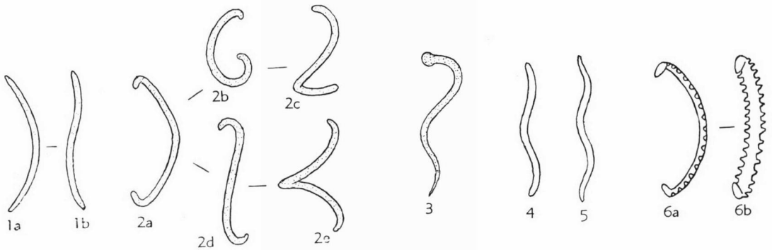
FIG. 5. Sigmaspires and variants from spicules of species of Craniella SCHMIDT and Chrotella SOLLAS.
