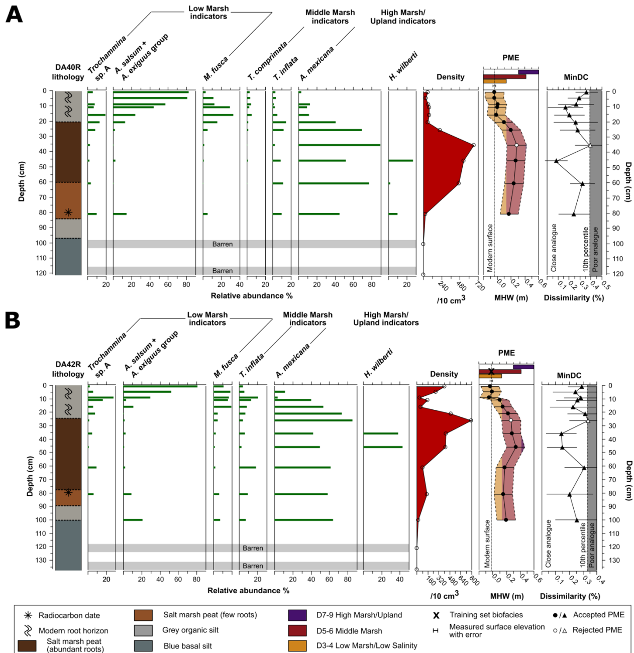
Figure 3.5. Stratigraphy, foraminiferal abundance, foraminiferal density, and Paleo-Marsh Elevation reconstruction with MinDC validation for core DA40R (A) and DA42R (B). Foraminiferal elevation optimum is ascending from left to right. Note that DA40R does not have a training set biofacies assigned due to census counts below the threshold for cluster analysis biofacies classification (Haller et al., in review; Chapter 2).
