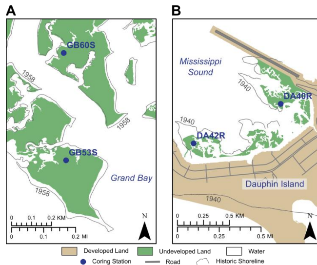
Figure 3.12. Modern salt-marsh extent compared with historic shorelines (grey contours). (A) Grand Bay: modern shoreline (2010) from Nelson et al. (2018), historic shoreline (1958) provided by Terrano et al. (2017). (B) Dauphin Island: modern (2015) shoreline (2015) and historic shoreline (1940) from Henderson et al. (2017).
