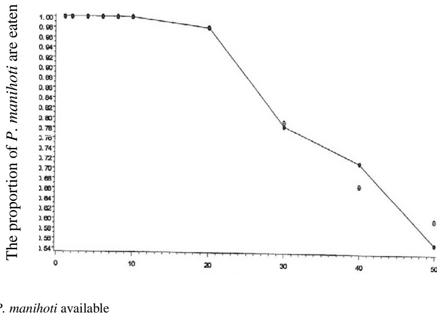
Figure 7. The average proportion of prey eaten at several densities prey
