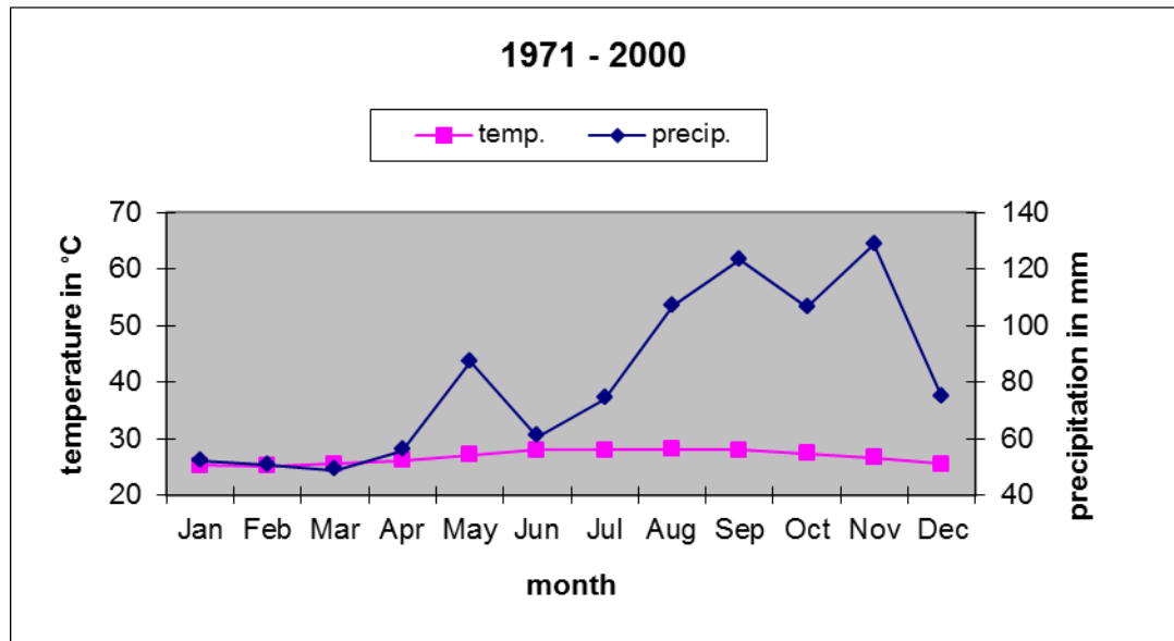
Figure 2 Walter climate diagram for the island of St. Eustatius (period 1971-2000; courtesy of: Meteorological Department Curaçao)
