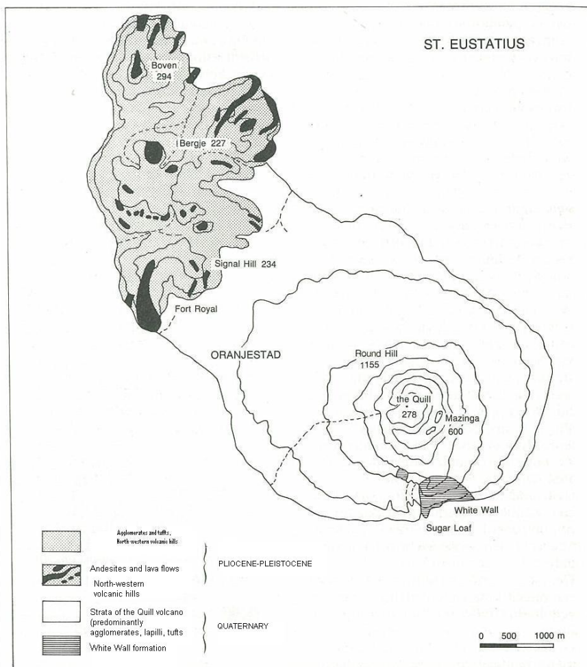
Geological map of St. Eustatius
