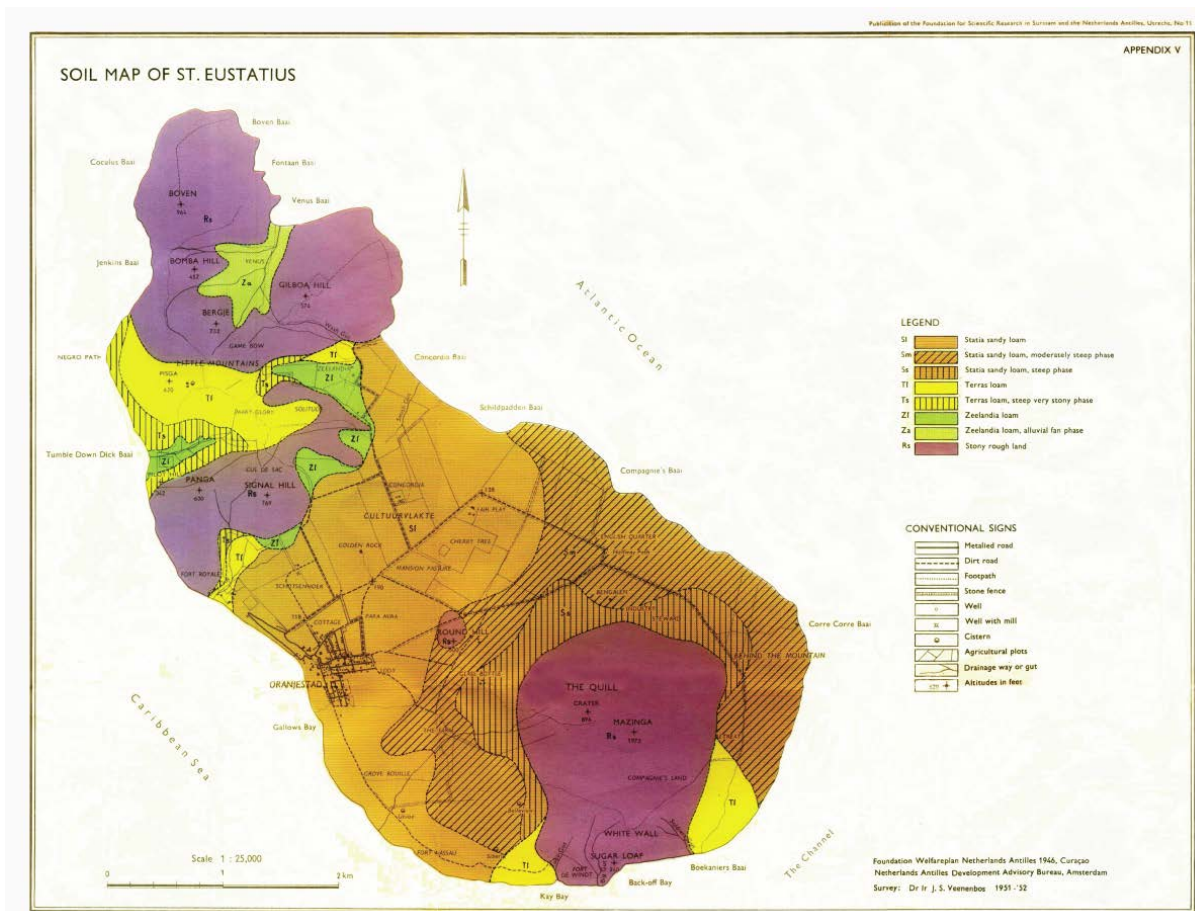
Figure 4 Soil map of St. Eustatius (source: Veenbos 1955).
